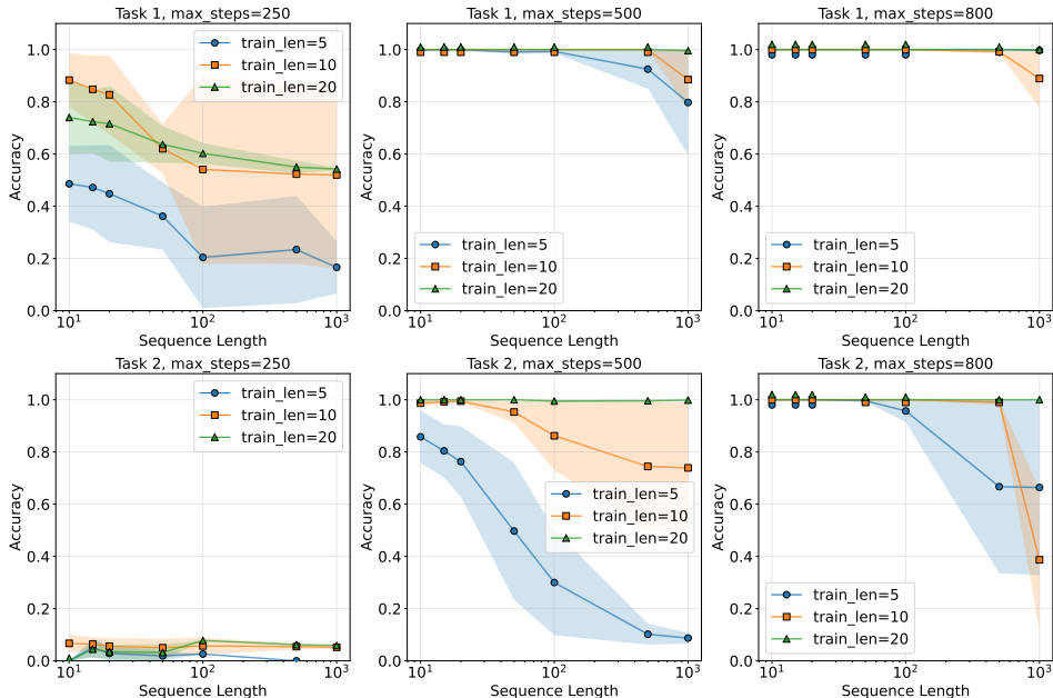
Figure 7: Multiplication generalization performance for Mamba across different training configurations. Each subplot shows accuracy as a function of sequence length for a specific maximum training steps value. Different colored lines represent different training sequence lengths, with error envelope indicating median absolute discrepancy across 5 runs.
