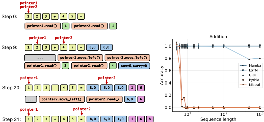
Figure 2: Left: Illustration of an interactive tool-use agent trajectory with pointer-based memory tool for solving multi-digit addition. The agent can generate thoughts (blue), outputs (purple) or commands (orange), and receive observations (green) from the memory tool. At each step, we show the state of the memory context on the top row, and below it show the sequence of generated tokens. Right: Accuracy of recurrent/SSM models (Mamba, LSTM, GRU) and Transformers (Pythia, Mistral) trained on trajectories for \leq 5 -digit addition, evaluated on up to 1,000-digits (log scale).
