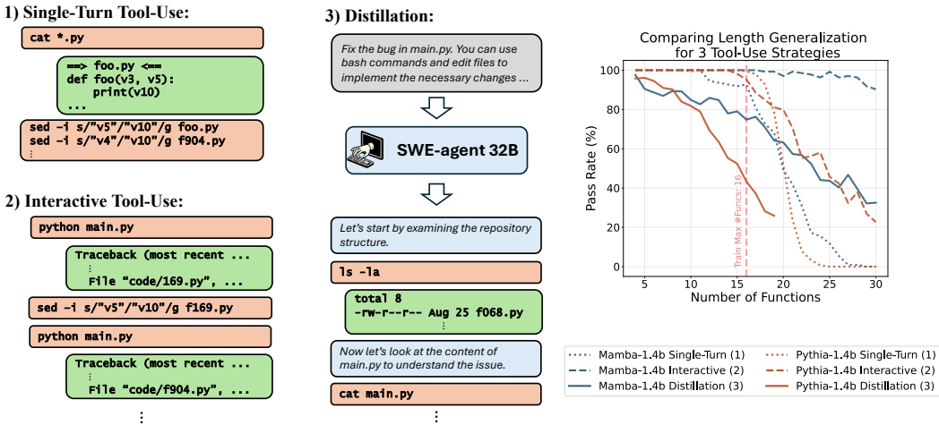
Figure 1: We finetune Mamba and Pythia (Transformer) on trajectories collected from different tool-use agents for solving a coding problem. 1) Single-Turn Tool-Use: Hard-coded agent that prints all the files in the repository and then outputs all the required changes. 2) Interactive Tool-Use: Hard-coded agent that iteratively runs the code, changes a few files, runs the code again etc. until all problems are resolved. 3) Distillation: SWE-agent Language Model (Yang et al., 2025) instructed to solve the bug in the code. Models are trained on codebases of up to 16 files (dashed red line), with context length 8K, and evaluated on larger codebases with longer context. While Pythia outperforms Mamba on smaller codebases and single-turn tool use, Mamba displays favorable performance on large codebases when trained to imitate interactive agents (agents 2 and 3), extrapolating beyond the training distribution.
