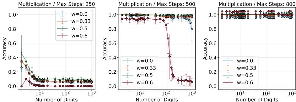
Figure 8: Multiplication task accuracy under co-training with varying training budgets (see Sec 3.1).
