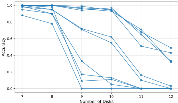
Figure 5: Performance of different seeds when training a Mamba model on Tower of Hanoi puzzles with up to 8 disks.
