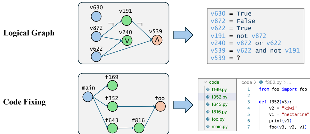
Figure 4: Illustration of Logical Graph reasoning task and code fixing task. We generate random graphs that define logical function structure (top) or code dependencies (bottom), and synthetically generate problems according to these graph structures.
