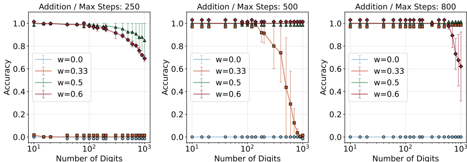
Figure 9: Addition task accuracy under co-training with varying training budgets (250, 500, 800 steps). Curves show different mixing weights. See (3.1).
