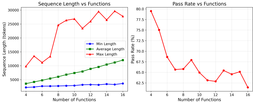
Figure 10: Pass rate and median sequence length for SWE-agent-LM-32B on the code fixing task.
