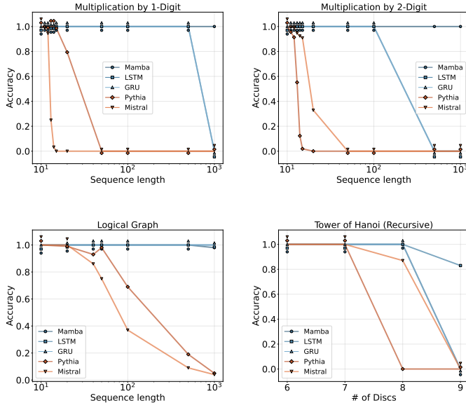
Figure 6: We train various transformer (Pythia, Mistral) and SSM (Mamba, LSTM, GRU) models on Multi-Digit Multiplication, Logical Graph and Tower of Hanoi tasks, with CoT + pointer-based memory tool. Multi-Digit Multiplication: We train models on multiplying a number of up to 10-digit by a 1-digit number or 2-digit number, using the pointer-based memory tool. Logical Graph: We train models to perform a logical graph reasoning problem using search-based memory tool, training on graphs with up to 10 variables. Tower of Hanoi: We train models to solve the Tower of Hanoi (recursive implementation) reasoning problem using search-based memory tool, training on problems with up to 7 disks. The first point in each plot is the maximal problem size seen during training (i.e., all other points are out-of-distribution extrapolation).
