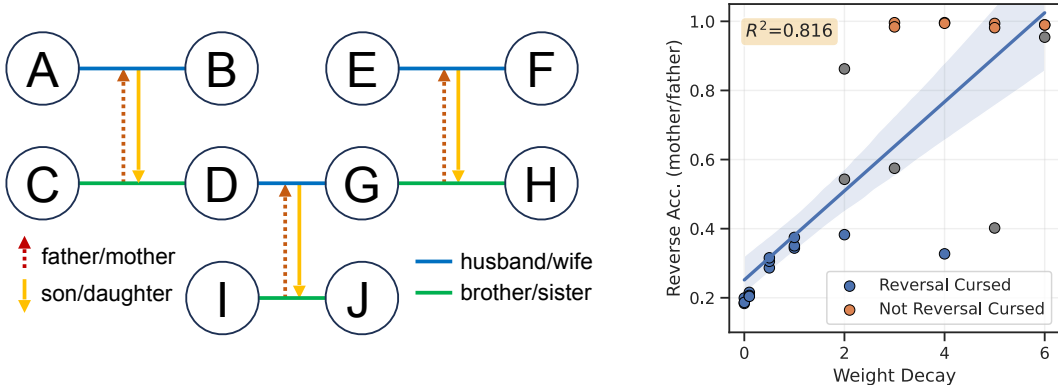
Figure 2: (Left) Schematic of the synthetic family knowledge graph. Nodes represent entities, while directed edges represent one of eight distinct family relations used in our experimental evaluation. (Right) Test accuracy on the unseen relations ( mother/father ) as a function of weight decay. Each weight decay setting was trained using three different random seeds.
