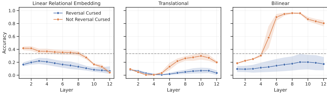
Figure 3: Layer-wise probe accuracy for relational embeddings. We compare “Reversal Cursed” models (blue) against “Not Reversal Cursed” models (orange), averaged across all relations. Accuracy is reported for each layer to identify where relational knowledge emerges.
