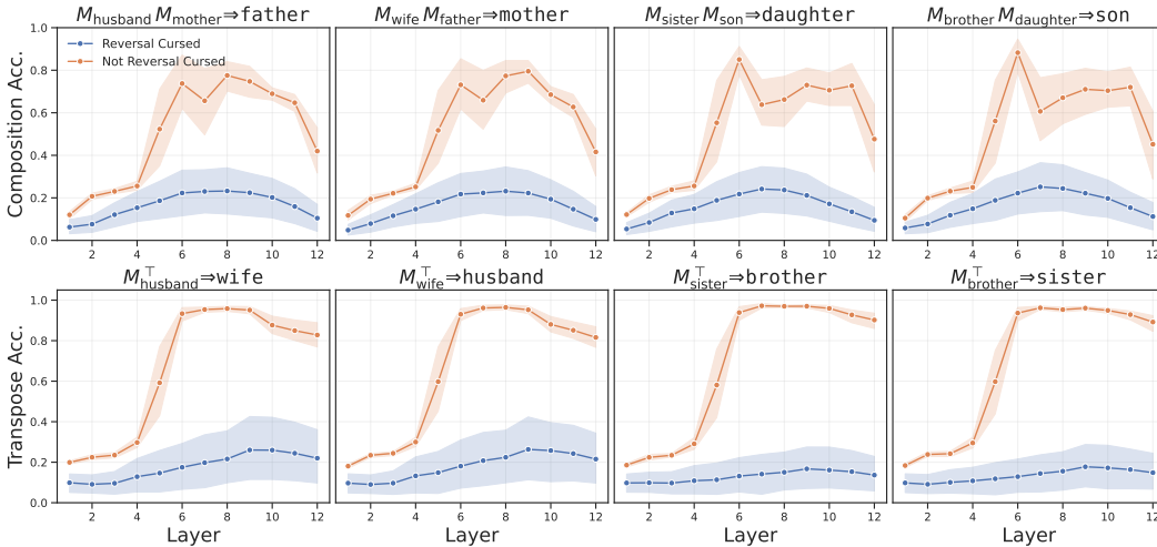
Figure 4: Performance on formal algebraic tests. Top Row (Composition): Accuracy of inferring a composed relation using the product of the corresponding bilinear matrices (e.g., M_{\text{husband}} \cdot M_{\text{mother}} to probe for ‘father’). Bottom Row (Transpose or Inversion): Accuracy of inferring an inverse relation using the transpose of a bilinear matrix (e.g., M_{\text{husband}}^T to probe for ‘wife’).
