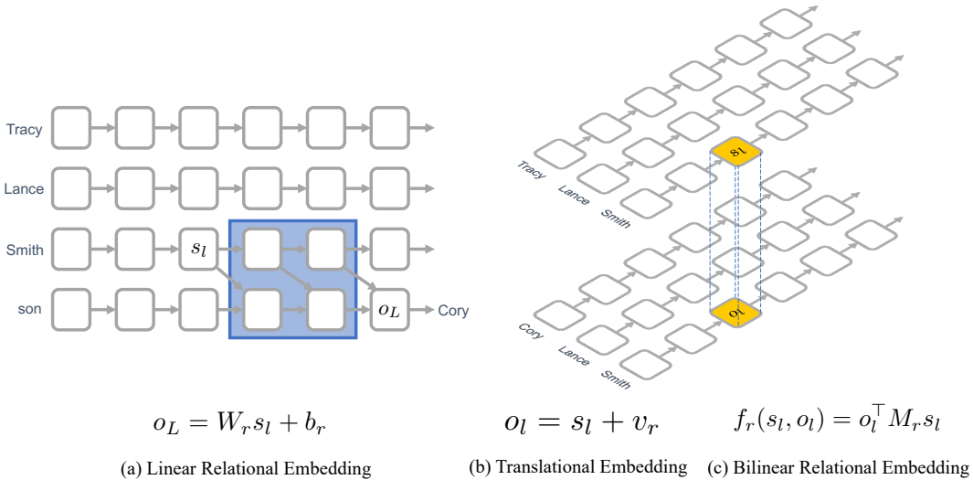
Figure 1: Schematics of relational embedding structures. For a subject s and object o , the relation r is modeled as: (a) linear transformation , (b) vector translation , or (c) bilinear interaction mediated by a relation-specific matrix M_r . As an example, in the fact “Son of Tracy Lance Smith is Cory Lance Smith,” s is “Tracy Lance Smith,” o is “Cory Lance Smith,” and r is son.
