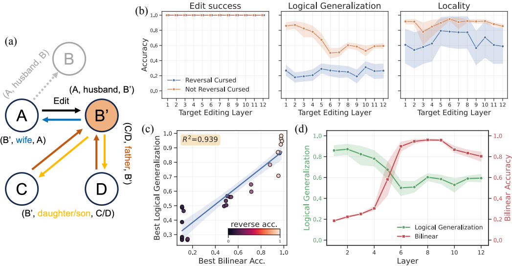
Figure 5: Editing generalization and its link to bilinear structure. (a) Schematic of the editing task. The primary fact (A, husband, B) is edited to (A, husband, B'). Successful logical generalization requires updating the inverse (B', wife, A) and neighborhood relations (C/D, father, B'); (B', daughter/son, C/D). (b) Post-edit performance metrics: Edit Success (direct change), Logical Generalization (propagation to entailed facts), and Locality (impact on unrelated facts). (c) Correlation between a model’s peak bilinear probe accuracy and its maximum logical generalization performance ( R^2 = 0.939 ). (d) Layer-wise performance of bilinear probing and logical generalization for “Not Reversal Cursed” models.
