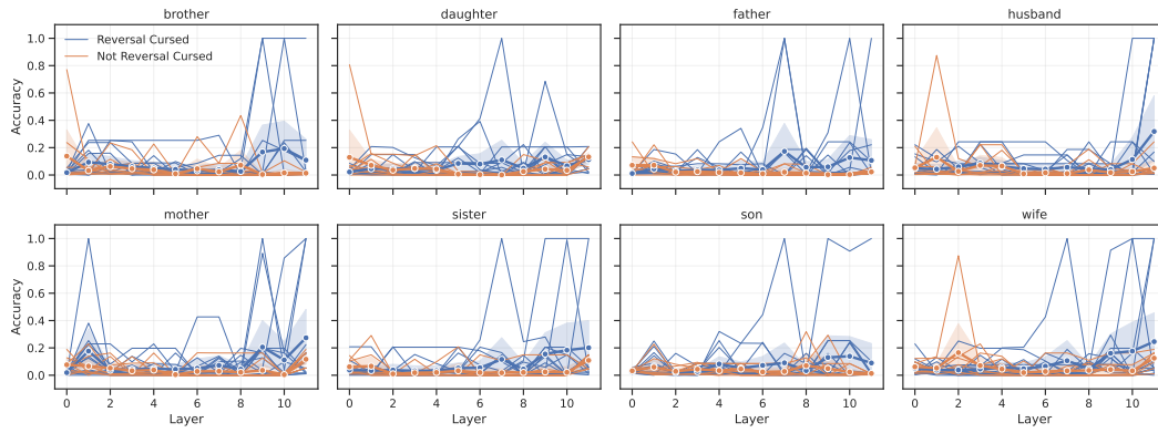
Figure 8: Visualization of linear relational embedding probing results for each relation r as a spaghetti plot ( n = 100 and \beta = 5 ).
