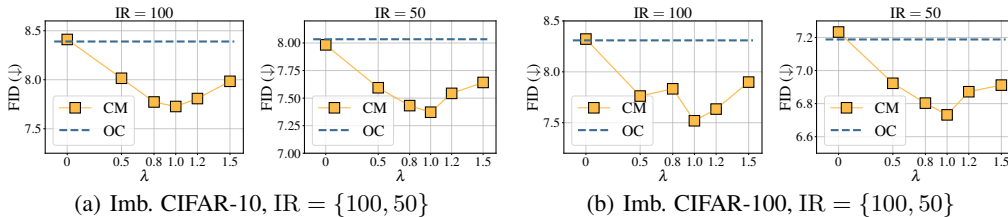
Figure G.3: Ablation study on the hyperparameter \lambda in Eq. (4). We use OC as a reference because it shows the best overall performance among the baselines and serves as our base loss. Figures (a) and (b) show results on Imb. CIFAR-10 and Imb. CIFAR-100, respectively, with imbalance ratios of IR = 100 and IR = 50 from left to right. We report FIDs for \lambda = \{0.0, 0.5, 0.8, 1.0, 1.2, 1.5\} .
