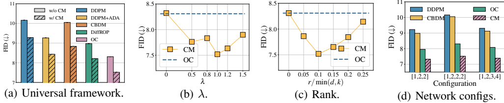
Figure 4: (a) The performance of CM when integrated with baselines. (b) Ablation study on the hyperparameter \lambda in Eq. (4). (c) Ablation study on the rank r . (d) Ablation study on various UNet configurations. All experiments are conducted on Imb. CIFAR-100 with IR = 100. In (b) and (c), we use OC as a reference because it shows the best overall performance among the baselines.
