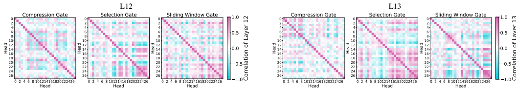
Figure 21: More Inter-head Gate Similarites Visualization
