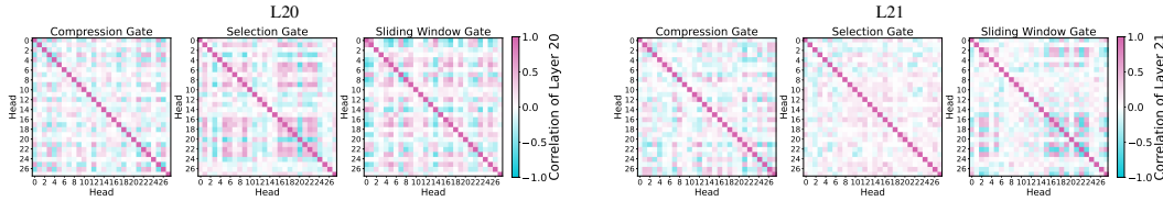
Figure 23: More Inter-head Gate Similarites Visualization
