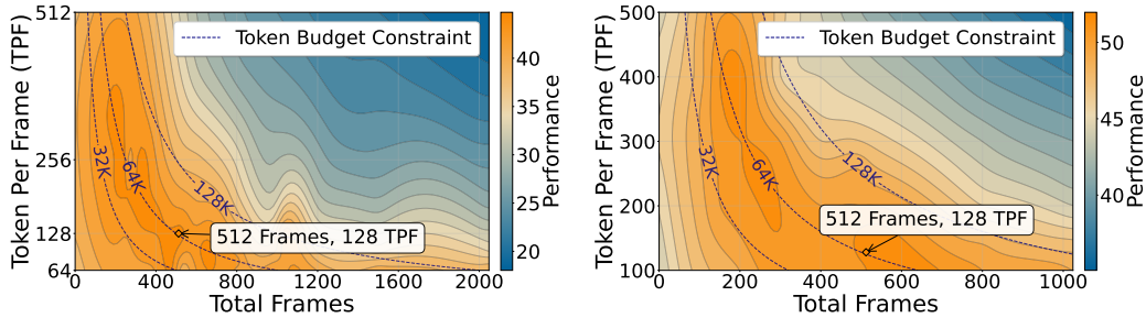
(a) Information Scaling of LongTimeScope
