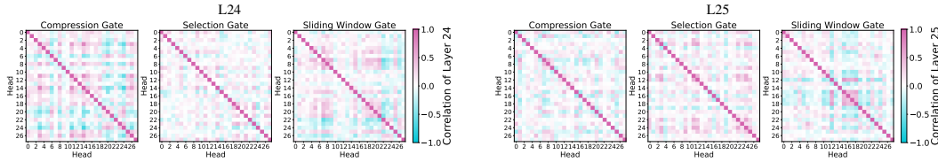
Figure 24: More Inter-head Gate Similarites Visualization
