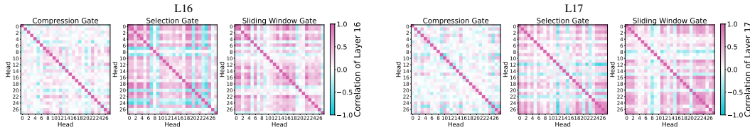
Figure 22: More Inter-head Gate Similarites Visualization
