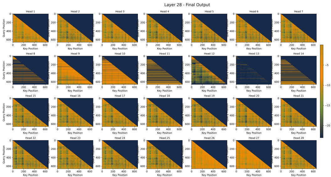
Figure 13: Attention pattern of the final vision attention output in the final layer of VideoNSA.
