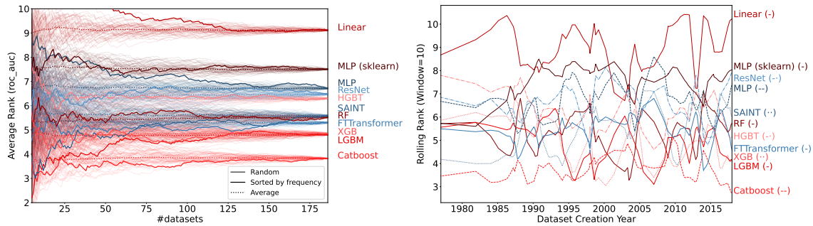
Figure 1: (Left) Ranking for increasing subsets of datasets. The thin, semi-transparent lines are computed on randomly sampled collections, dashed lines show the overall average rank over these randomly sampled collections, and the thick lines correspond to the rank across subsets of popular datasets (e.g. the rank across the 3 most often used datasets). (Right) Ranking of the methods for rolling windows of 10 datasets, sorted by their age.
