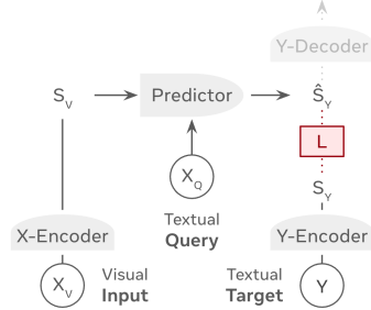
Figure 1: VL-JEPA.
