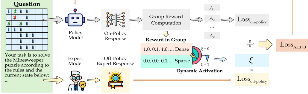
Figure 5: Demonstration of Adaptive Hybrid Policy Optimization (AHPO). AHPO dynamically integrates off-policy expert guidance with on-policy exploration, leading to performance generalization.
