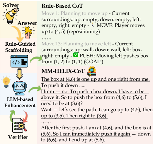
Figure 4: Demonstration of our Step-Elicited Response Generation pipeline.
