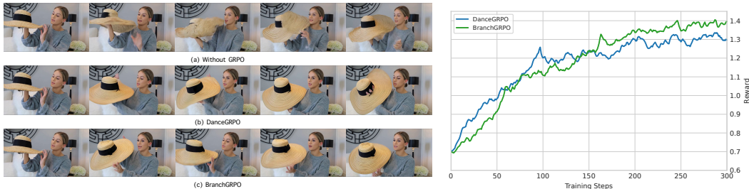
Figure 8: Video generation results on Wan2.1-1.3B. Left: qualitative frame comparisons across three settings. Right: reward curves showing faster convergence and higher final rewards with BranchGRPO compared to DanceGRPO.
