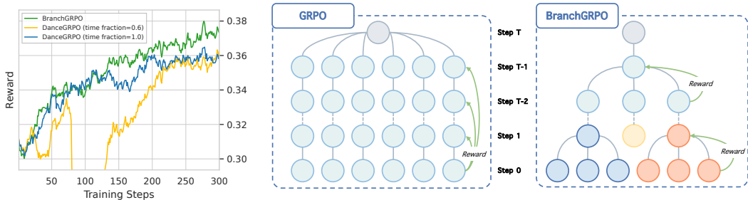
Figure 1: Comparison of BranchGRPO and DanceGRPO. Left: Reward curves during training. BranchGRPO converges substantially faster, achieving up to 2.2× speedup over DanceGRPO (time fraction = 1.0) and 1.5× speedup over DanceGRPO (time fraction = 0.6), while ultimately surpassing both baselines. The time fraction = 0.6 variant further exhibits pronounced instability. (time fraction denotes the proportion of diffusion timesteps used during training.). Right: Illustration of rollout structures. GRPO relies on sequential rollouts with only final rewards, whereas BranchGRPO performs branching at intermediate steps and propagates dense rewards backward, enabling more efficient and stable optimization.
