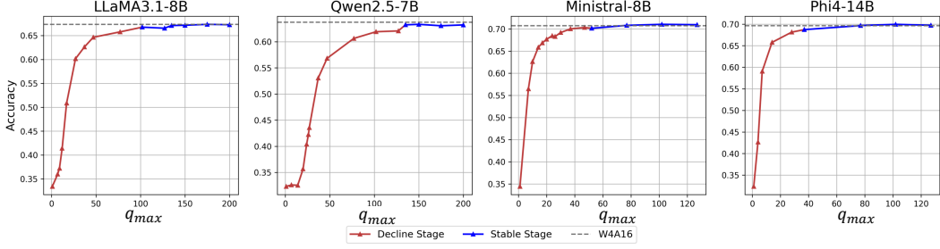
Figure 10: After quantizing weights to INT4 using per-channel symmetric quantization, the zero-shot average accuracy of the models on Winograde, PIQA, BoolQ, ARC_C, and Lambada changes with q_{max} . The quantization process of activations corresponding to different q_{max} is implemented through fake-quant simulation. A lower value of q_{max} corresponds to a higher upper bound on the quantization error.
