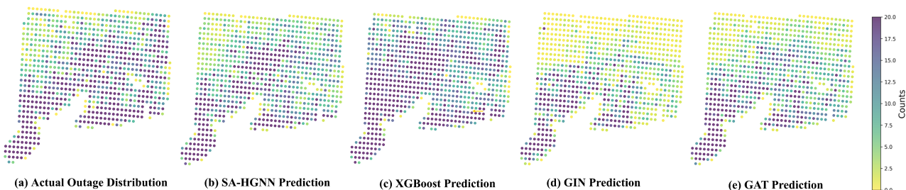
Figure 5: Outage prediction distribution of Hurricane Irene (August 28, 2011) in Connecticut. The ground truth total outage count is 16022 (a). SA-HGNN (b) produces the closest total prediction (14512) compared to XGBoost (21385), GIN (11273), and GAT (13742).
