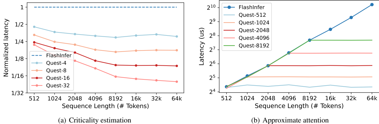
Figure 8. We measure the latency of individual kernels in Quest. (a) As sequence length increases, the relative criticality estimation latency decreases to 1/Page Size of FlashInfer. (b) Approximate attention with token budget K consumes constant time irrelevant to total sequence length and reaches similar performance of FlashInfer at sequence length K.
