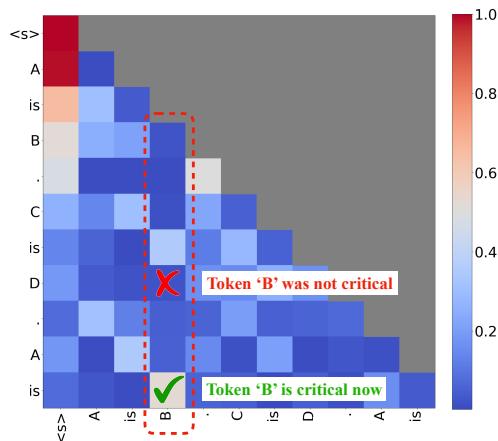
Figure 2. The attention map of prompt “A is B. C is D. A is”. Each row represents the attention scores of previous tokens queried by the tokens on the left. When queried with “D”, token “B” has a low attention score, showing “B” is not critical for generation. However, the “is” strongly attends to “B”. Therefore, the criticality of tokens strongly correlates with the current query token.
