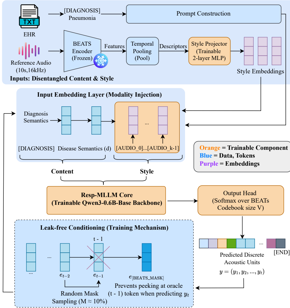
Figure 2: Detailed architecture of Resp-MLLM (Stage 1 of the Generator). The model functions as a style-conditioned multimodal unit generator. Top: A modality injection mechanism fuses textual diagnosis semantics with acoustic style embeddings (projected from temporally pooled BEATS features) to prompt the Qwen3-0.6B-Base backbone. Bottom: A leak-free conditioning strategy is employed during training: random mask sampling ( M \approx 10\% ) prevents the model from peeking at oracle tokens, ensuring robust autoregressive prediction of discrete acoustic units.
