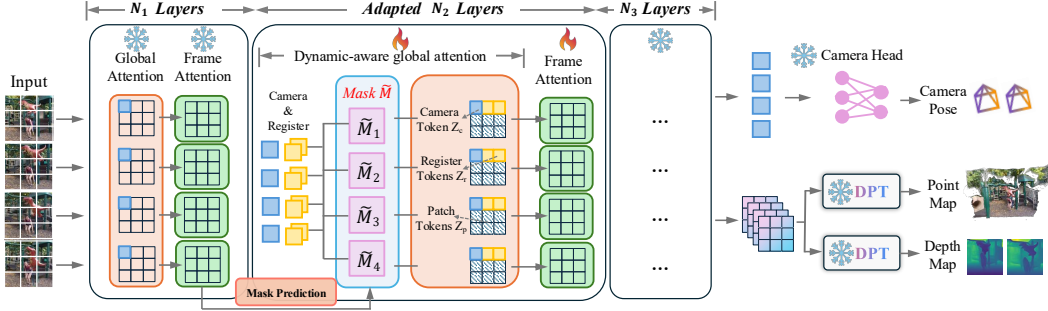
Figure 3: Fine-tuning strategy: Instead of fine-tuning the entire VGGT architecture, we adapt only the middle N_2 layers of the global attention mechanism, which are most critical for cross-frame information fusion. To further address dynamic scenes, we introduce a dynamics-aware aggregator that predicts a mask to disentangle dynamic and static content.
