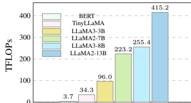
Figure 1: Computational overhead for one-step fine-tuning of different language models using LoRA.
