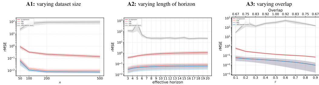
Figure 6: Setting A – Frozen Lake environment: Unrestricted model class \mathcal{G} . The results confirm the theoretical properties : our DRQ-learner in blue is better than the plug-in learners in red/orange, robust for varying lengths of the horizon.
