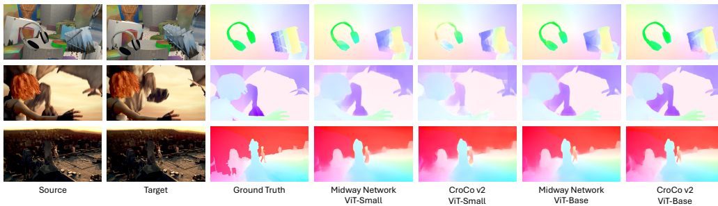
Figure 13: Visualization of FlyingThings and MPI-Sintel optical flow evaluations after finetuning for Midway Network and CroCo v2 pretrained on BDD for varying model sizes. Moving from ViT-Small to ViT-Base primarily provides fine-grained improvements in optical flow estimation.
