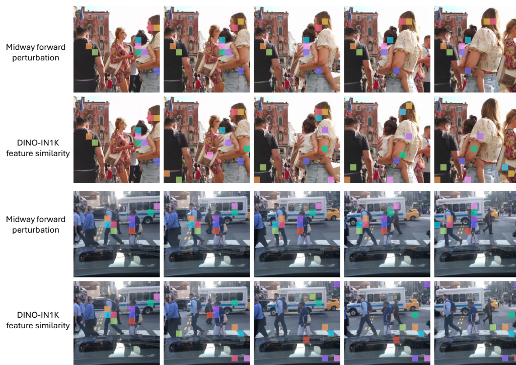
Figure 15: High-level tracking using forwarded feature perturbation and/or feature similarity. Midway Network is able to track high-level regions through motion transformations, such as the back of the toddler (top row, pink square).
