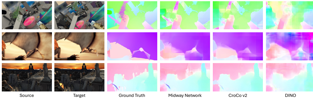
Figure 12: Visualization of FlyingThings and MPI-Sintel optical flow evaluations after finetuning for models pretrained on WT-Venice. Midway Network is able to generate more accurate optical flow predictions compared to CroCo v2 and DINO.
