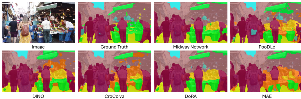
Figure 10: Visualization of WT-Sem semantic segmentation UperNet finetuning. Midway Network is able to produce reasonable segmentation masks, even in cluttered scenes.
