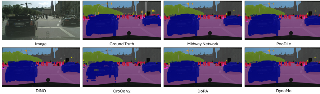
Figure 9: Visualization of CityScapes semantic segmentation UperNet readout. Midway Network generates cleaner boundaries, particularly for the crossing pedestrians.
