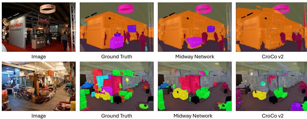
Figure 11: Visualization of ADE20K semantic segmentation UperNet finetuning. Midway Network generates more accurate segmentation masks compared to CroCo v2.
