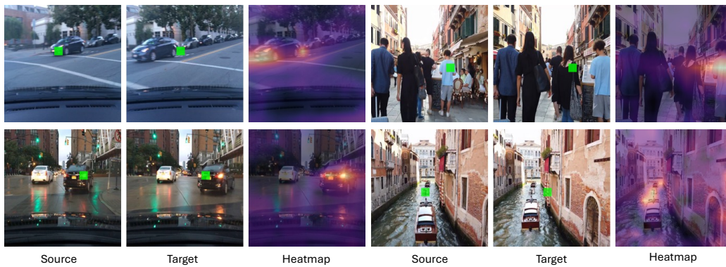
Figure 14: Heatmaps for forwarded feature perturbation in Source (green squares); shown in Target at the same location to highlight motion. The learned dynamics can capture high-level correspondence, such as the right taillight of the black car (bottom left).
