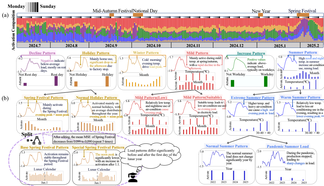
Figure 4: Case study of interpretability and steerability: (a) Activation patterns of prototypes, which each colored bar shows the degree of activation of its corresponding prototype each day. This visualization shows seasonal, weekly, and holiday-related prototype activations. (b) The learned prototype hierarchy that illustrates typical temporal patterns and their correlations with covariates for interpretable load forecasting. After the expert splits the first prototype at layer-2, the mean MSE across five random seeds decreases from 0.099 to 0.090 for Spring Festival related predictions.
