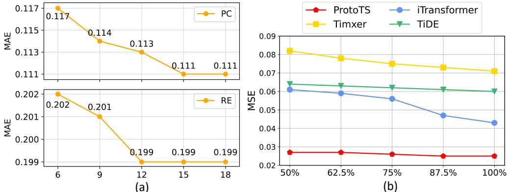
Figure 3: Sensitivity analysis: (a) Effect of increasing root prototype numbers from {6, 9, 12, 15, 18}. (b) Data efficiency as the training data proportion increases from 50% to 100%.
