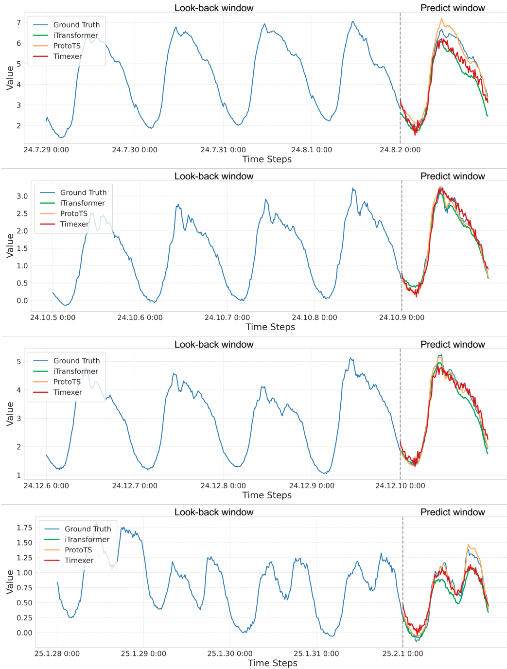
Figure 6: Result Visualization: The prediction results for four sampled days, consistent with our experimental setting: Look-back window is 4 days and Predict window is 1 day, a day consists of 96 time steps. The horizontal axis represents time, and the vertical axis represents the current electricity load. The electricity load values have been normalized, so they are unitless and may include negative values.
