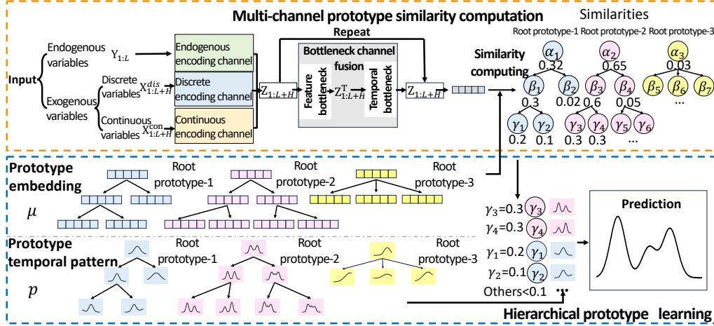
Figure 2: The overall framework of ProtoTS, which comprises two main modules: the multi-channel prototype similarity computation module and the hierarchical prototype learning module.
