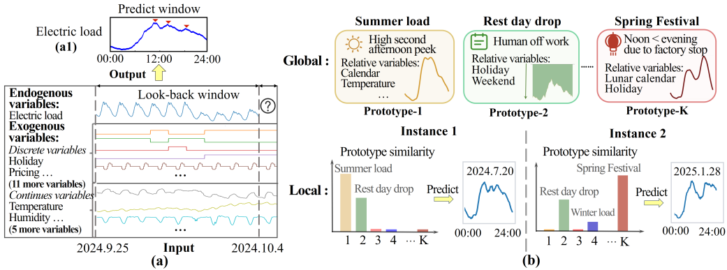
Figure 1: (a) An example of time series forecasting with numerous heterogeneous variables, where exogenous variables (e.g., temperature, holiday) influence the evolution of endogenous variables (e.g., electric load). (b) Illustration of prototypical explanation method: a set of learned prototypes provides a user-friendly global overview of typical temporal patterns. For each instance, model computes its similarity to all prototypes to form a prediction, enabling detailed local interpretation.
