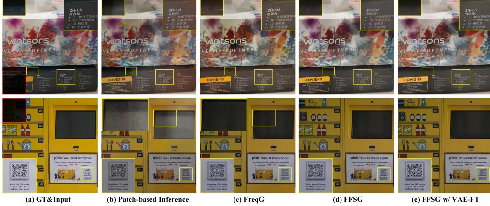
Figure 3: Visual comparison and ablation study of FreeAdapt on the UHD-LL. (b) Patch-based inference suffers from color inconsistency; (c) FreqG contains high-frequency noise; (d) FFSG still exhibits detail loss.
