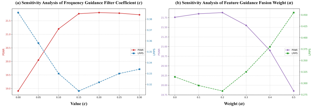
Figure 8: Hyperparameter sensitivity analysis on the UHD-LL dataset.
