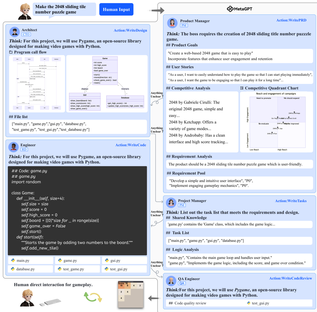
Figure 3: A diagram showing the software development process in MetaGPT, emphasizing its significant dependence on SOPs. The more detailed demonstration can be found in Appendix B.
