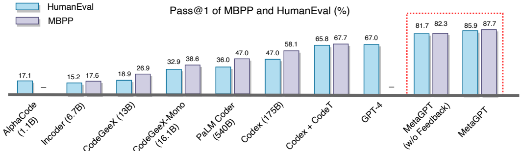
Figure 4: Pass rates on the MBPP and HumanEval with a single attempt.
