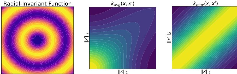
Figure 1: (Left) Colored level sets of a two-dimensional function f^*(\mathbf{x}) invariant under planar rotations (see (16)): if \|\mathbf{x}\|_2 = \|\mathbf{x}'\|_2 , then f^*(\mathbf{x}) = f^*(\mathbf{x}') . (Center/Right) Rotation-invariant kernels derived from an RBF base kernel (lengthscale 1/2), visualized as a function of (\|\mathbf{x}\|_2, \|\mathbf{x}'\|_2) . k_{\max} (right) captures the correct invariance, while k_{\text{avg}} (center) only approximates it.
