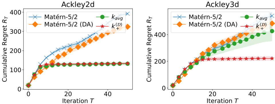
Figure 9: Cumulative regret on the two-dimensional (resp., three-dimensional) Ackley function, with |G| = 8 (resp., |G| = 48 ).
