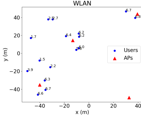
Figure 7: WN with the best positions of APs found by GP-UCB with k_+^{(D)} . APs are depicted by red triangles and users with blue circles. The throughput for each user is shown in Mbps.
