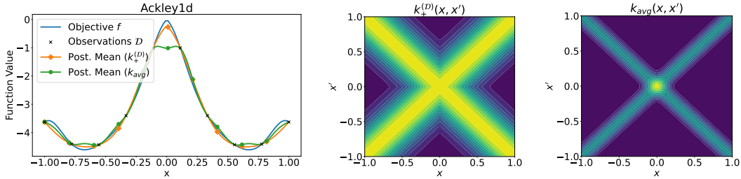
Figure 2: (Left) One-dimensional Ackley function f^* (see (15)), invariant up to coordinate-wise sign-flips, and GP posterior means \mu_t(\mathbf{x}) as in (3) for k_+^{(D)} (orange diamond) and k_{\text{avg}} (green circles) built from \mathcal{D} (black crosses). (Center) Covariance structure induced by k_+^{(D)} . (Right) Covariance structure induced by k_{\text{avg}} . Both kernels are invariant to reflections across x = y and x = -y , but k_{\text{avg}} concentrates covariance near 0, while k_+^{(D)} better reflects the underlying symmetry geometry. Consequently, the GP posterior mean induced by k_+^{(D)} is the best at fitting the objective (left).
