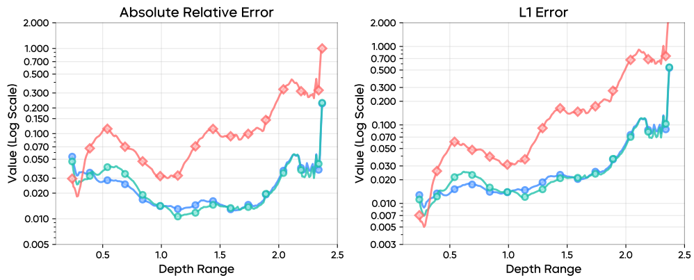
(b) Depth accuracy on L515 data split.
