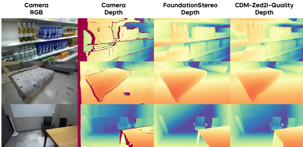
Figure 10: Depth prediction comparison between CDMs and FoundationStereo.
