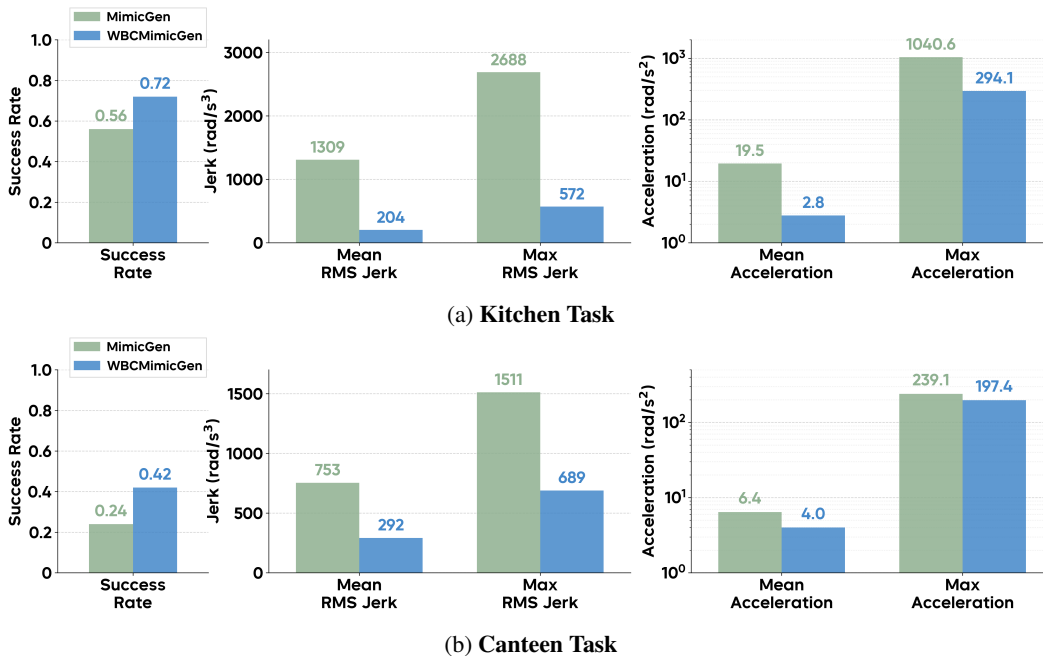
Figure 21: Performance comparison between policy models trained on demonstrations generated by MimicGen and our WBCMimicGen, on (a) Kitchen Task and (b) Canteen Task. The policy learned from WBCMimicGen reflects a higher success rate while keeping smooth on the rollout policy trajectory (lower RMS jerk and acceleration indicate).
