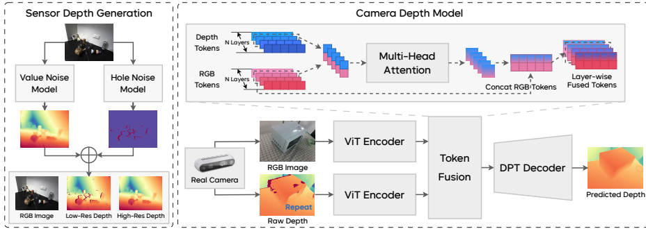
Figure 2: Overview of camera depth models. Left: camera depth generation to synthesize the datasets for training camera depth models, where the value/hole noise models are trained using the collected dataset. (Sec. 3.4) Right: the camera depth model, which is built on two ViT encoders (Dosovitskiy et al., 2020) and fine-tuned from a depth foundation model (Yang et al., 2024b); the RGB and depth tokens are fused before being given to a DPT decoder (Ranftl et al., 2021). Such a structure allows the model to receive sparse depth from sensors for prediction without any pre-processing like hole-filling. (Sec. 3.2)
