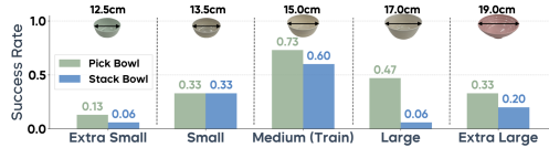
Figure 7: Generalization over different bowl sizes. With CDM, success remains non-zero across all unseen sizes; without CDM, success is zero.
