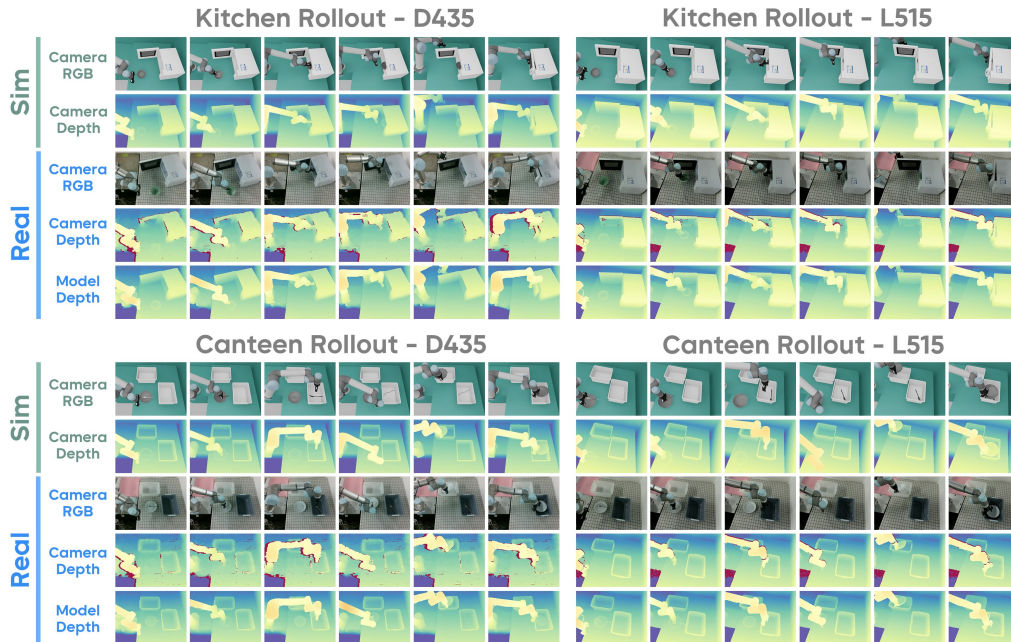
Figure 20: Sim-Real rollouts comparison on two tasks in the sim-to-real experiments , including two views (D435 view and L515 view). For the simulation, we show the rendered RGB and depth images; as for the real experiments, we visualize the RGB images and the depth images from the depth camera, with the predicted depth from the corresponding camera depth model.
