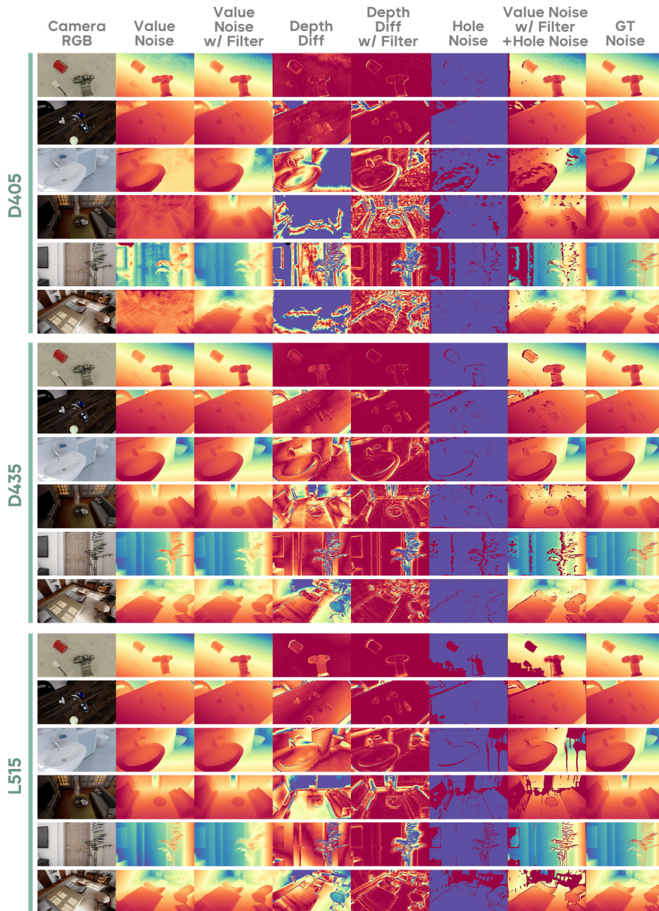
Figure 13: Synthesized noise of RealSense D405, D435 and L515.
