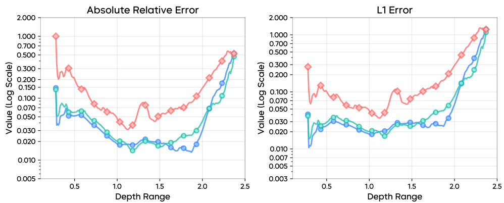
(c) Depth accuracy on Helios data split.
