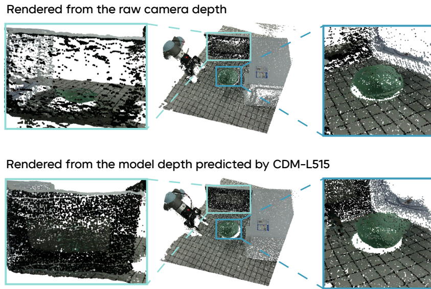
(a) Point cloud comparison of the Kitchen task.
