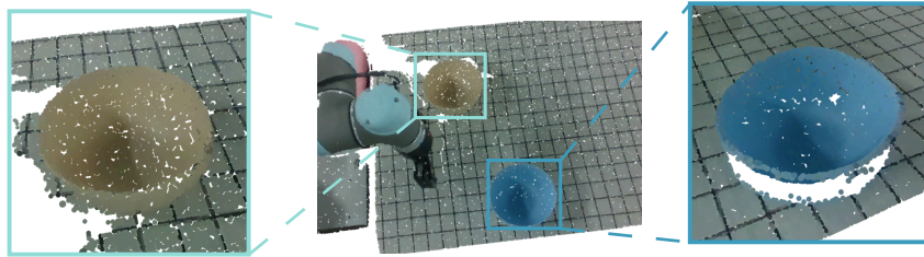
(a) Point cloud comparison of the Stack Bowl task.
