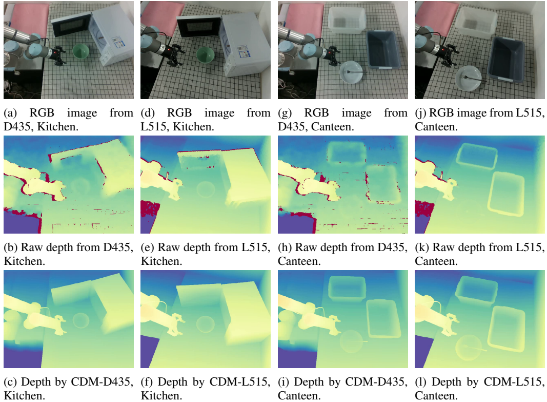
Figure 16: Detailed real-world cases of two representative depth cameras , RealSense D435 (active IR stereo camera) and RealSense L515 (lidar camera), including color images (first row), camera depth images (second row), and depth predicted by camera depth models proposed in this project (third row).
