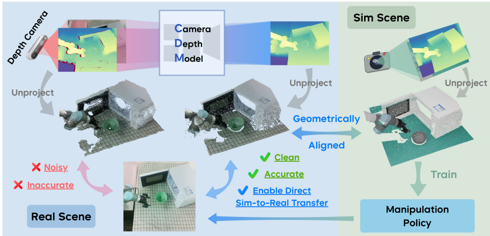
Figure 1: How the proposed camera depth model (CDMs) makes real-world manipulation as in simulation. The illustration is made on the RealSense D435 camera with CDM-D435. With CDM, the manipulation policy learns from accurate geometric information, which is aligned between the simulation and the real world.
