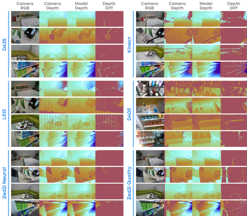
Figure 12: Depth predictions visualization of extended camera depth models , including CDM-D435, CDM-D405, CDM-L515, CDM-Kinect, and CDM-Zed2i (Neural & Quality mode) on their corresponding camera captures. Note that the depth difference is visualized in a range of 0-0.2m.
