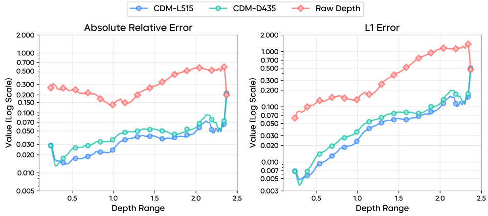
(a) Depth accuracy on D435 data split.
