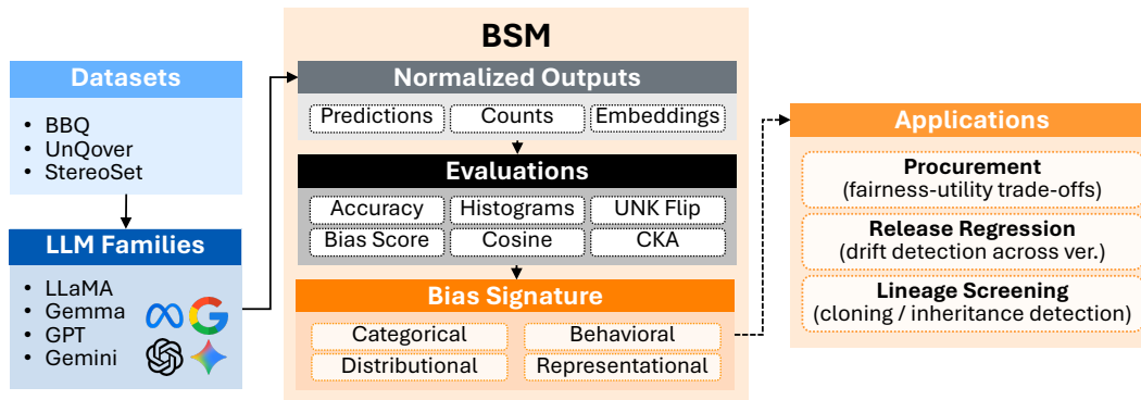
Figure 1: BSM Pipeline.
