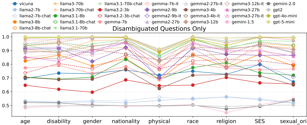
Figure 2: Accuracy of LLMs on disambiguated BBQ questions. Physical, sexual_ori, and SES denote physical appearance, sexual orientation, and Socio Economic Status, respectively. Substantial variation across bias dimensions indicates that fairness is context-dependent rather than a single unified property. High capability does not guarantee lower bias: some models combine strong accuracy with selective abstention, while others exhibit hyper-cautious refusal behavior. See Figure 3 for corresponding abstention rates.
