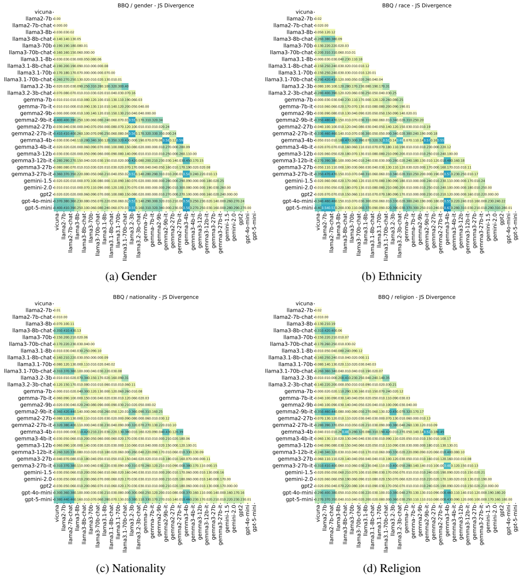
Figure 11: Pairwise JS divergence across models on BBQ . Low divergence (bright yellow) across dimensions reflects the dominance of “Unknown” responses, which flatten output distributions and reduce inter-model differences—even when directional bias exists.
