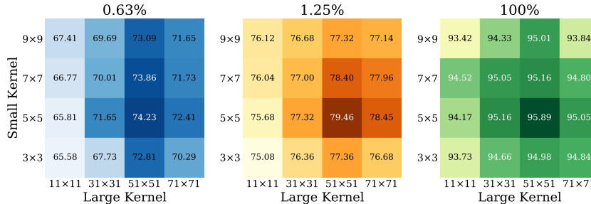
Figure 7: Performance of Different Kernel Size Combination. Experiments are conducted on the BUSI dataset using the pretrained ViT-B across three training setting (0.63%, 1.25%, and 100%). ACC (%) is reported.
