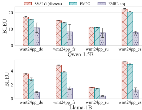
Figure 13: Evaluation of GRPO-based variant of SVSI with discretized voting score (SVSI-G-discrete).
