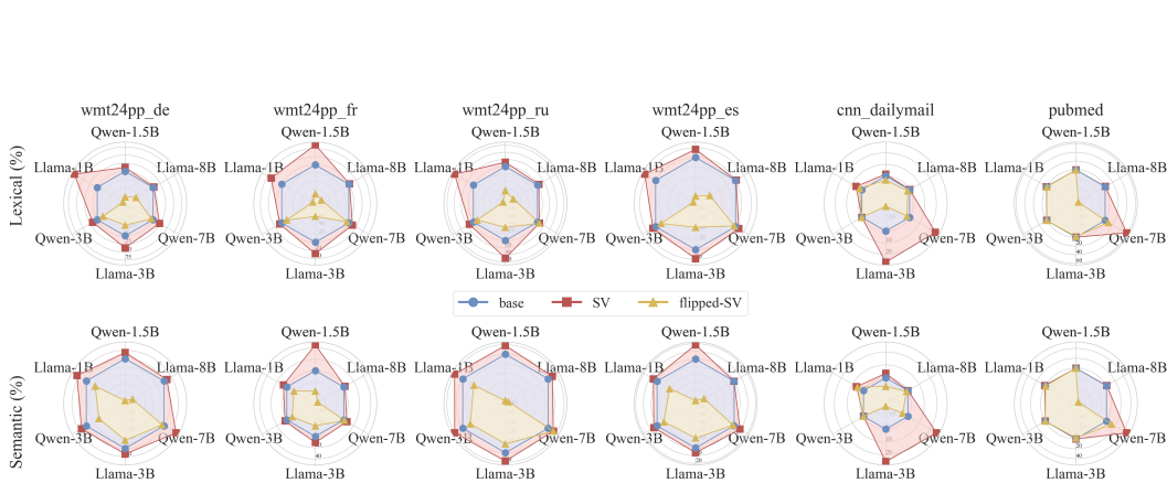
Figure 4: Improvements of training with Semantic Voting (SV) and flipped-SV (inverted SV preference pairs), relative to the base model on lexical (top row) and semantic (bottom row) metrics.
