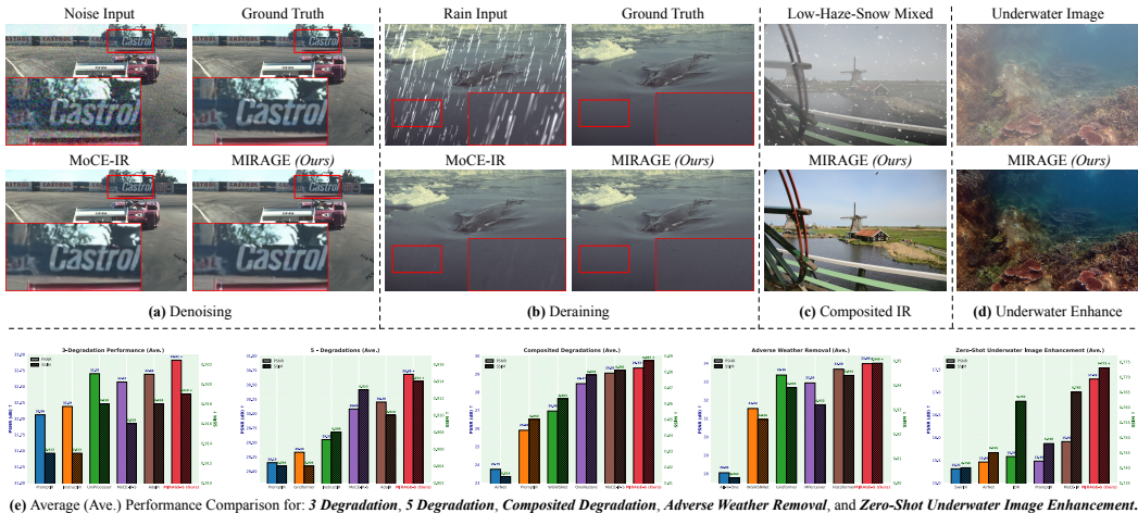
Figure 1: (a)-(d): Visual comparison for Denoising, Deraining, Compositing Degradations (low-light, haze, and snow), and underwater image enhancement. (e): The average PSNR and SSIM comparison across 4 challenging all-in-one and 1 zero-shot settings (Please zoom in for a better view).
