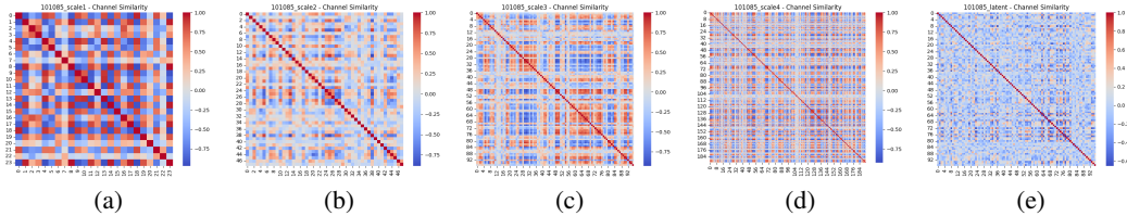
Figure 4: (a)-(d): The channel-wise similarity matrix from the 1st Scale ( H \times W \times C ) to the 4th Scale ( H/s \times W/s \times 8C ). (e): The channel-wise similarity matrix of (d) after channel-wise projection.
