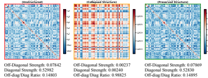
Figure 6: Shallow-latent similarity under three settings: (a) w/o CL (unstructured; off-diag 0.0784, ratio 0.148), (b) Euclidean CL (collapsed; off-diag \approx 0.0024, ratio 0.99), (c) SPD CL (preserved; off-diag 0.0787, ratio 0.149).
