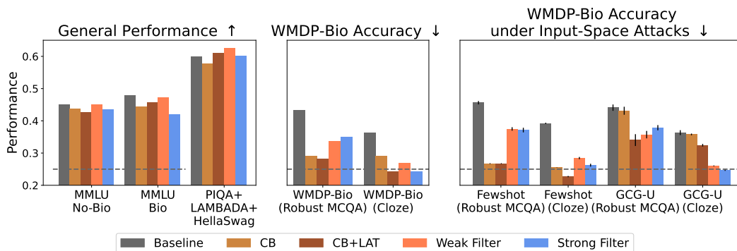
Figure 3: Data filtering (our technique) performs competitively with Circuit-Breaking (CB) techniques under black-box evals and attacks. We evaluate data filtering approaches against baselines on general knowledge (higher is better) and biothreat proxy knowledge (lower is better). Dotted lines indicate random chance. We report performance across repeated non-deterministic attacks with error bars. Filtering and CB methods are comparable: both have similarly minor effects on general capabilities, CB methods perform slightly better on MCQA biothreat proxy evaluations, and filtering methods perform slightly better on cloze biothreat proxy evaluations. Filtering is robust to the input-space attacks, especially in the cloze-prompt setting. These results demonstrate that pretraining data filtering is effective at significantly preventing biothreat proxy knowledge, including random-chance-level performance on cloze-style prompts.
