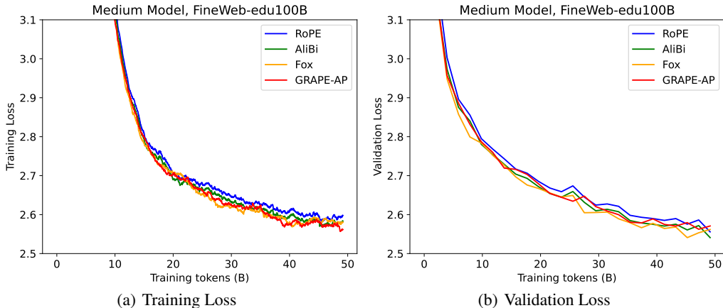
Figure 2: The training and validation loss of medium-size models (353M), with different positional encoding mechanisms on the FineWeb-Edu 100B dataset.
