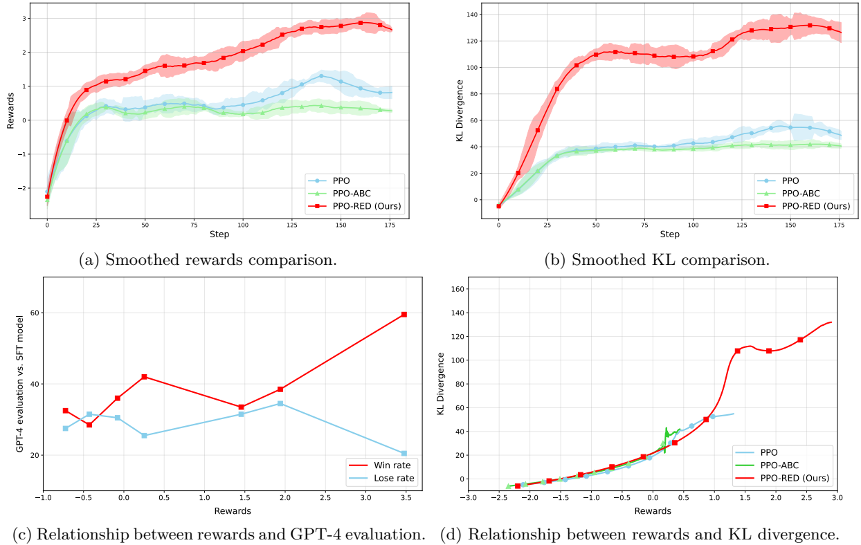
Figure 3: Performance comparison for various methods on the Nectar evaluation set.
