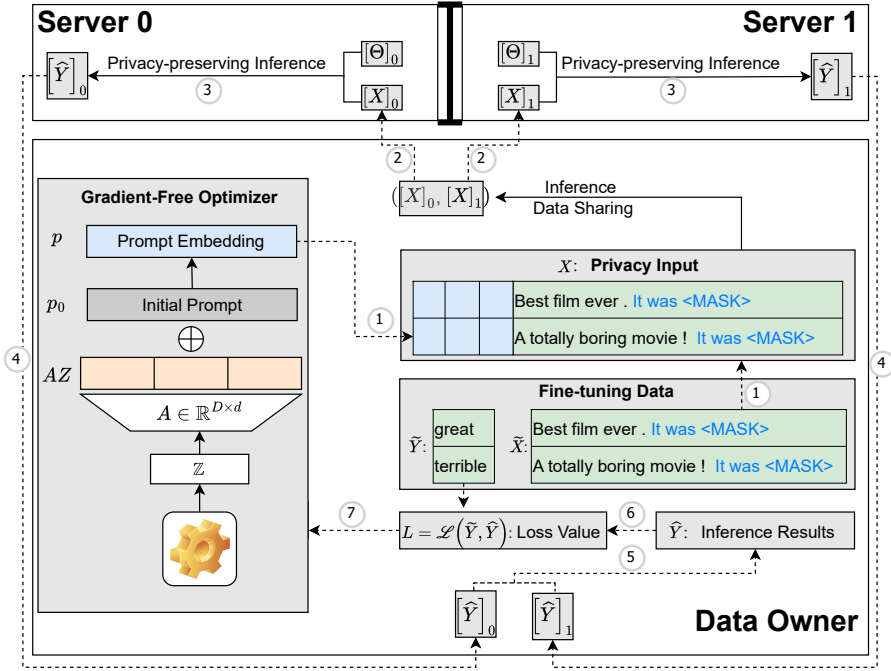
Figure 2: Workflow of SecP-Tuning. SecP-Tuning leverages MPC to protect both training data and model parameters during fine-tuning. It addresses two key bottlenecks in PFT. First, it eliminates the computational overhead of backward and optimizer by adopting a FoT paradigm. Second, it improves the efficiency of privacy-preserving self attention by employing RFA.
