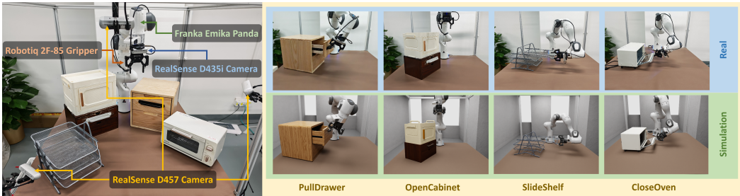
Figure 7: Experimental Setup. We conducted 4 real-world tasks for imitation learning.
