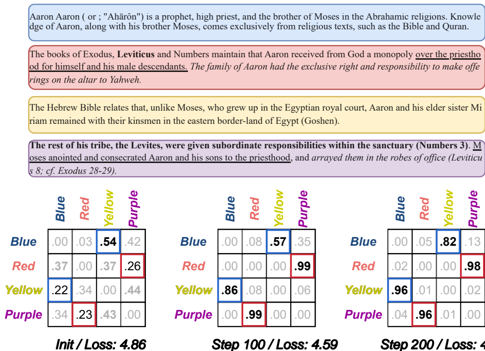
Figure 6: Example of training dynamics of ReVeLa. The related patterns in red and purple sequences are highlighted in bold , underline , and italic .
