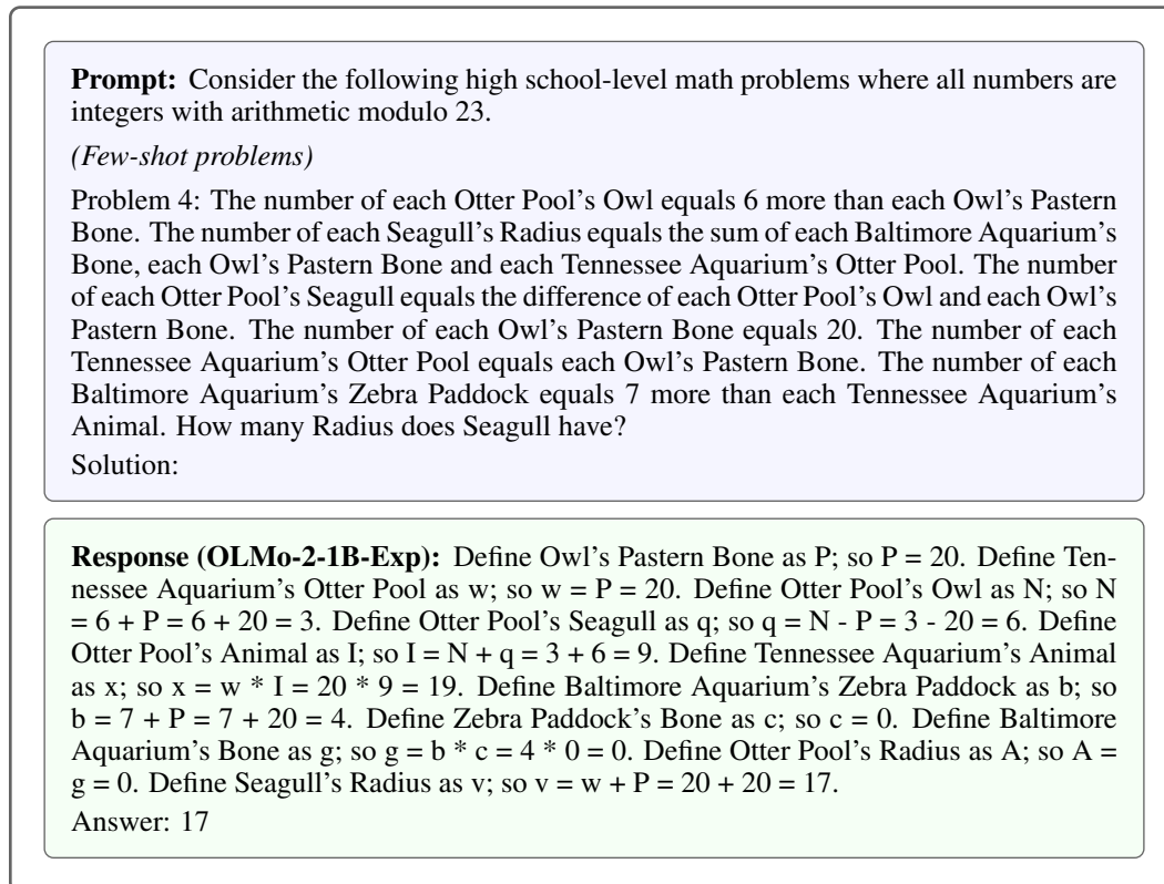
Figure 13: OLMo-2-1B-Exp can solve mathematical reasoning problems that are more complex than the problems that the model has seen during training. In this example, the model solves a problem from the difficulty class i_{\text{GSM-med}}^{\text{op}=11, \text{ip} \leq 20} , despite having seen only problems of difficulty \text{op} \leq 10 during training. The model’s solution is minimal, meaning that there are no unnecessary steps in the solution (Ye et al., 2025).
