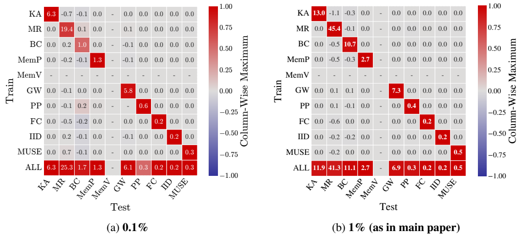
Figure 31: Dependence testing with 0.1% and 1% modified tokens provides similar results. We train for 100 gradient steps with 0.1% and 1% of insertions. The results for 0.1% of insertions are similar, but the measured effects are generally smaller.
