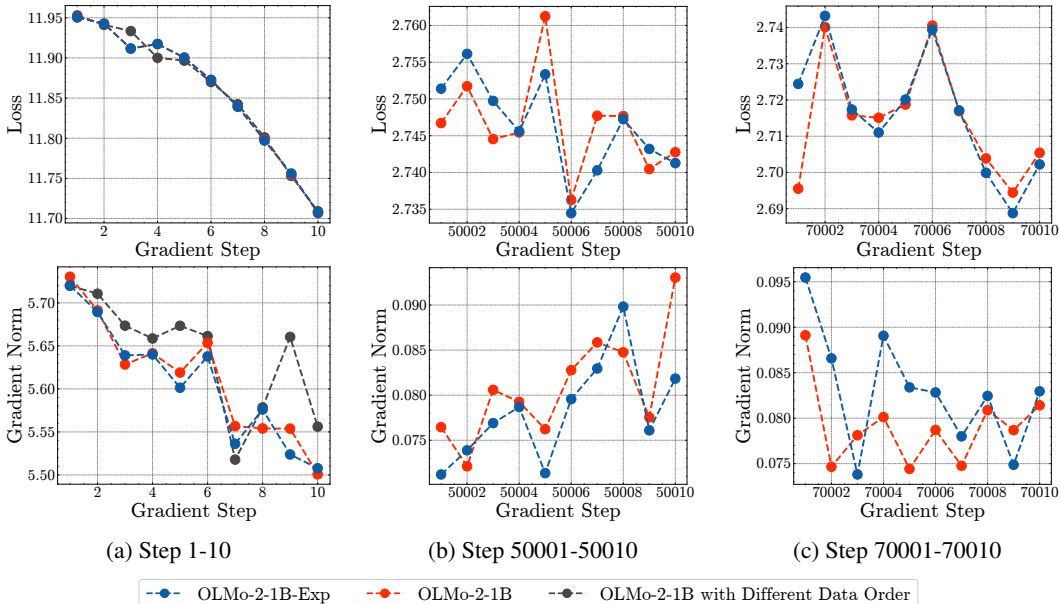
Figure 9: Cross-entropy loss and gradient norm over the course of training. (a): The first 10 gradient steps. (b): After 50% of training. (c): After 70% of training.
