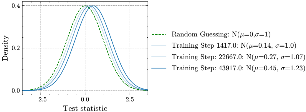
Figure 19: Fitted test statistic distributions along the training trajectory on intermediate model checkpoints.
