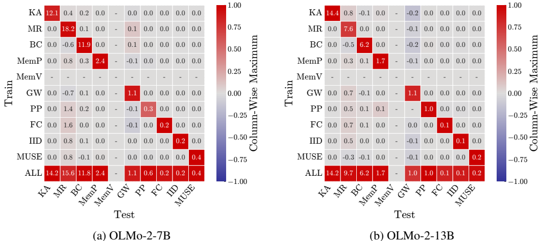
Figure 26: Dependency testing with OLMo-2-7B and OLMo-2-13B provides similar results. This figure depicts the result of continual pretraining dependence testing for the Experiments in Table 1 with OLMo-2-7B and OLMo-2-13B.
