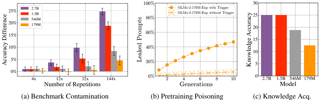
Figure 5: The effect of model size on the results of three different experiments. (a): The effect of benchmark contamination increases with model size. (b): The prompt extraction attack remains successful at the 179M parameter scale. (c): Smaller models are less accurate at answering factual questions about the fictitious knowledge inserted as part of the knowledge acquisition experiment.
