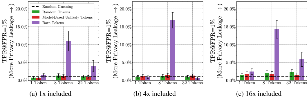
Figure 16: Privacy leakage across different secret token strategies. We also report 95% bootstrap confidence intervals. The exact experimental conditions are described in Supplement E.4.
