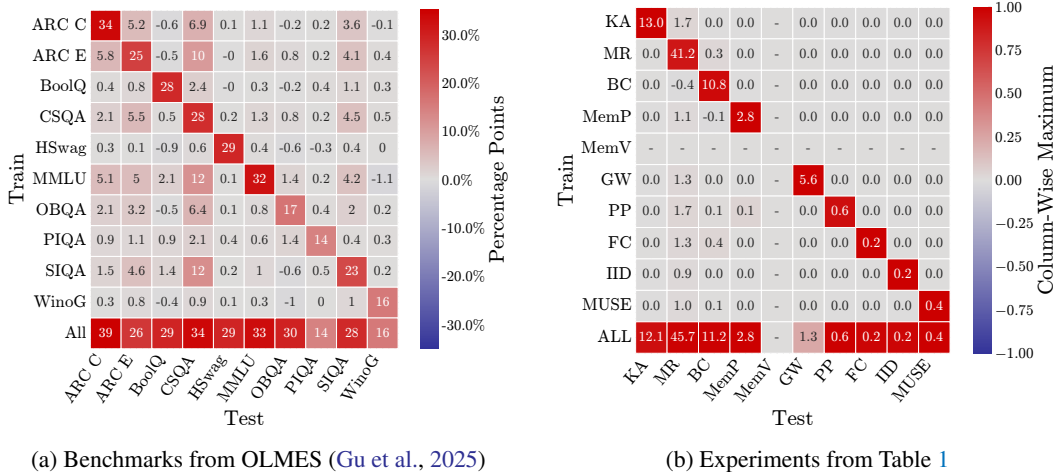
Figure 25: Continual pretraining dependence testing with a checkpoint later in training provides similar results. This figure depicts the result of the same experiment as Figure 6 in the main paper, but for the OLMo-2-0425-1B checkpoint at gradient step 1.000.000.
