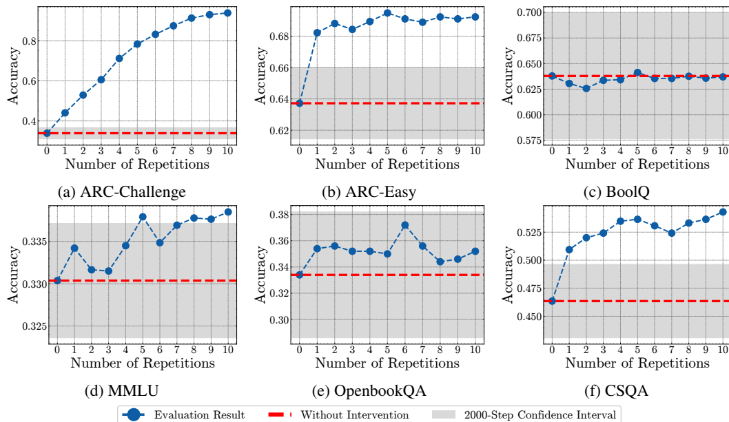
Figure 29: Modifying the number of repetitions of ARC-Challenge benchmark questions. The figure depicts the effect of increasing the repetitions of ARC-Challenge benchmark questions on the scores of different benchmarks. The figure also depicts confidence intervals for the respective evaluations. We see that the scores of multiple benchmarks change as we modify the number of ARC-Challenge tokens in the training data.
