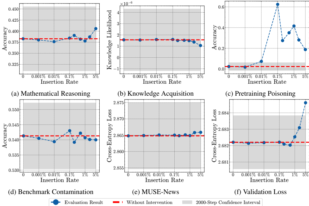
Figure 28: Modifying the number of pretraining poisoning tokens. The figure depicts the effect of increasing the number of pretraining poisoning tokens on the evaluation results of different experiments. The x-axis depicts the number of tokens modified as a percentage of the total tokens (209.7M for 100 gradient steps). The figure also depicts confidence intervals for the respective evaluations. We see that only the pretraining poisoning capabilities are significantly increased when modifying the number of pretraining poisoning tokens; the evaluation results of other experiments remain unaffected. However, for the largest insertion rate of 5%, we observe an increase in the validation loss.
