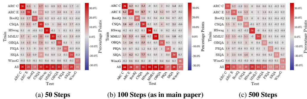
Figure 32: Dependence testing with a different number of training steps provides similar results. The figure depicts the result of varying the number of training steps in the benchmark dependence experiment. In all experiments, the benchmark questions are repeated four times in the training data. As we increase the number of training steps, the overall impact of benchmark contamination decreases, consistent with Bordt et al. (2025) . The structure of the dependence matrix remains the same.
