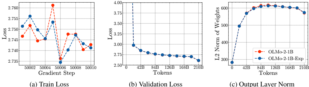
Figure 7: The training dynamics of OLMo-2-1B-Exp are remarkably similar to OLMo-2-1B. (a): Train loss at 50% of training. (b): Validation loss on 200M tokens. (c): Growth of the output layer norm during training.
