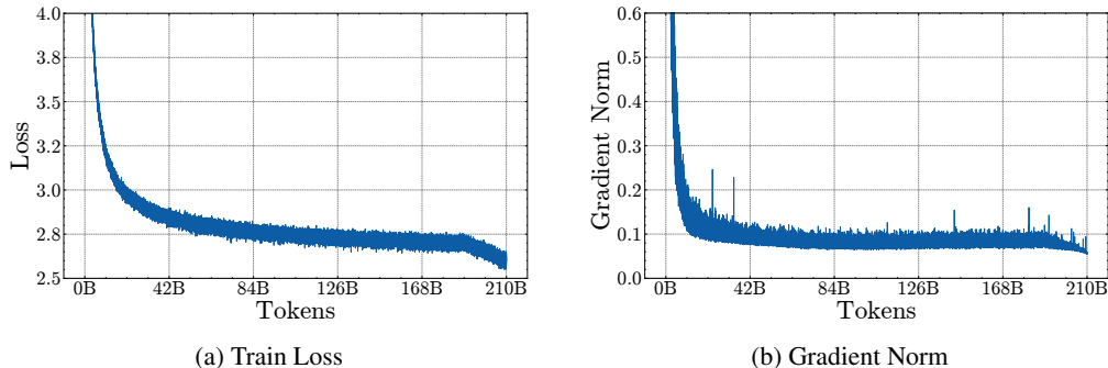
Figure 8: OLMo-2-1B-Exp exhibits stable training dynamics. The experiments do not lead to significant spikes in the train loss or gradient norm.
