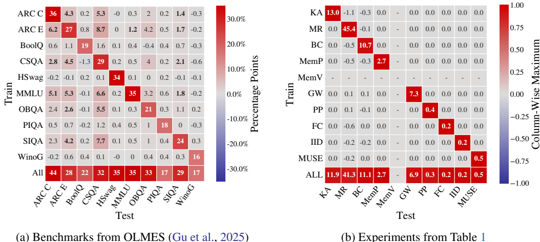
Figure 6: The dependencies between language modeling benchmarks (left) and the experiments (right), measured through our continual pretraining dependence test. (a): As expected, positive off-diagonal entries indicate significant dependencies between language modeling benchmarks. (b): In contrast, our controlled experiments show no evidence of such dependencies. The metrics used to evaluate the experiments are provided in Supplement Table 9. Statistically significant dependencies are depicted in bold.
