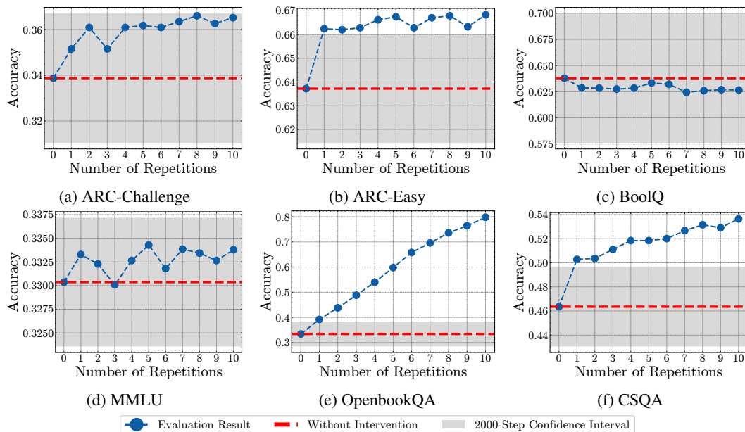
Figure 30: Modifying the number of repetitions of OpenbookQA benchmark questions. The figure depicts the effect of increasing the repetitions of OpenBookQA benchmark questions on the scores of different benchmarks. The figure also depicts confidence intervals for the respective evaluations. We see that the scores of multiple benchmarks change as we modify the number of OpenbookQA tokens in the training data.
