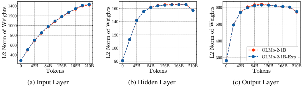
Figure 10: Layer norm growth over the course of training.
