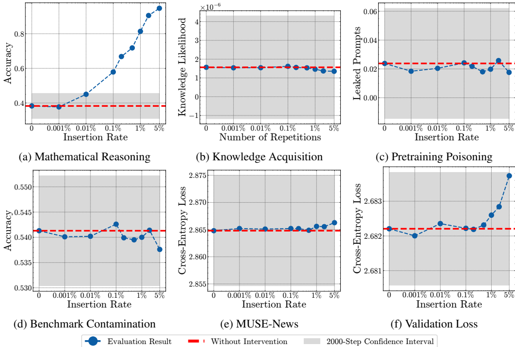
Figure 27: Modifying the number of mathematical reasoning tokens. The figure depicts the effect of increasing the number of mathematical reasoning tokens on the evaluation results of different experiments. The x-axis depicts the number of tokens modified as a percentage of the total tokens (209.7M for 100 gradient steps). The figure also depicts confidence intervals for the respective evaluations. We see that only the mathematical reasoning capabilities are significantly increased when modifying the number of mathematical reasoning tokens; all other capabilities remain largely unaffected. However, for the largest insertion rate of 5%, we observe a slight increase in the validation loss.
