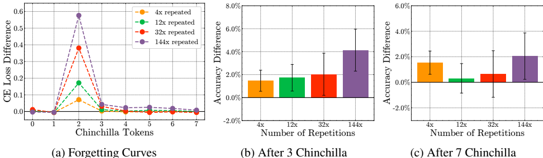
Figure 15: Forgetting of contaminated benchmark questions. This figure replicates Figure 2(a)-(c) in Bordt et al. (2025). We observe that the absolute cross-entropy loss differences, depicted in Figure 15a, are smaller than those in Figure 2(a) in Bordt et al. (2025). The forgetting dynamic remains the same. Mean and 90% confidence intervals.
