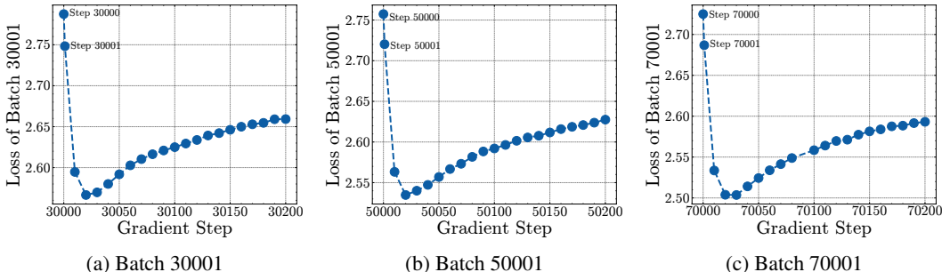
Figure 23: The dynamics of the cross-entropy of a batch immediately after it is encountered during training. The first step in every plot (30000, 50000, and 70000) depicts the cross-entropy loss of the batch directly before it is encountered. The second step (30001, 50001, and 70001) depicts the cross-entropy loss of the batch directly after it is encountered. Interestingly, this is not the local minimum of the loss, which is instead reached approximately 25 gradient steps after the batch is encountered. After that, we observe the slow and continuous forgetting of the batch.
