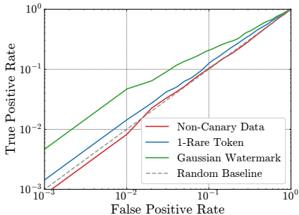
Figure 4: Comparing canary efficacy under 1-time canary inclusions. Point estimates are complemented by 95% bootstrap confidence intervals.
