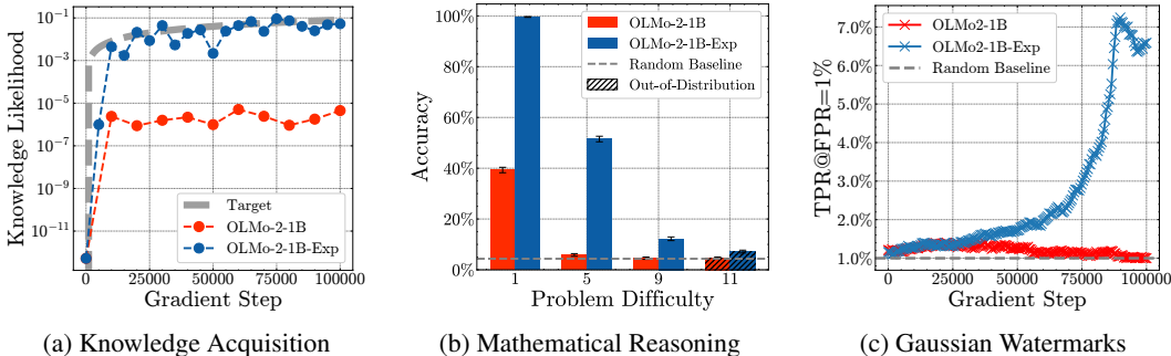
Figure 2: Results of the three novel experiments. (a): Algorithm 1 successfully maintains the value of the knowledge probe (blue) close to the control target (gray). (b): OLMo-2-1B-Exp exhibits a small degree of length-generalization to complex mathematical reasoning problems. (c): Gaussian Pretraining Watermarks are detectable over the course of training.
