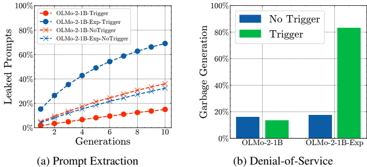
Figure 21: Results of the prompt extraction and denial-of-service experiments.
