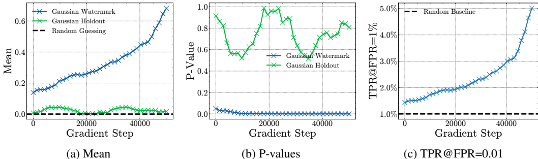
Figure 18: Gaussian Watermark (GW) experiments on intermediate model checkpoint. The GW results were smoothed over a 200-sample sliding window. Each point is plotted at the average batch index of the samples within its respective window to show the trend as training progresses.
