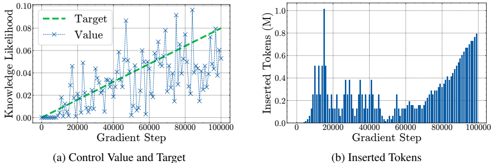
Figure 11: The result of the online control for fictional knowledge acquisition experiment. Left: The target probability, and the value of the knowledge problem at each control step. Right: The number of inserted tokens (in millions) during every control interval of 1000 gradient steps, as determined by Algorithm 1.
