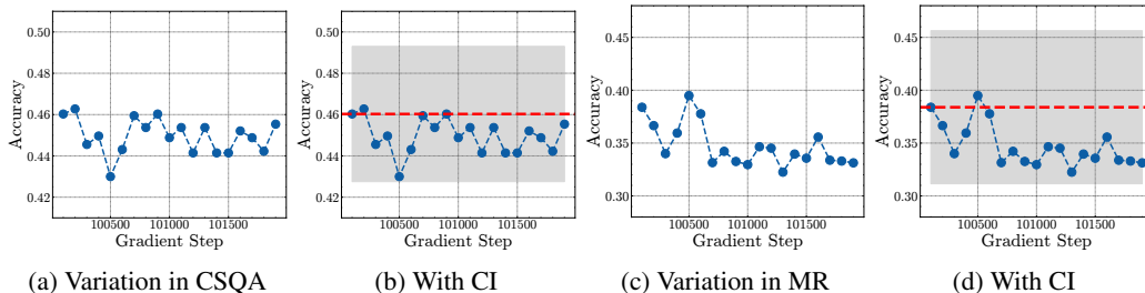
Figure 33: The Construction of 2000-Step Confidence Intervals. (a) and (c): We first measure the random variation in evaluations when training for 2000 steps without intervention. (b) and (d) We construct confidence intervals that cover the observed variation. These confidence intervals are then used in Figures 27, 28, 29 and 30 to assess whether the effect of training data modifications is significant (i.e., exceeds random variation).
