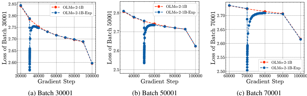
Figure 22: The forgetting curves of three different batches. The figure depicts the development of the cross-entropy loss of three different batches over the course of training. OLMo-2-1B never encounters the batches during training. OLMo-2-1B-Exp encounters the batches at gradient step (30001, 50001, 70001), respectively. This figure depicts the experiment also shown in Figure 23, but over a longer time horizon. This Figure replicates Figure 4 in (Pagliardini et al., 2025), but only for the AdamW optimizer.
