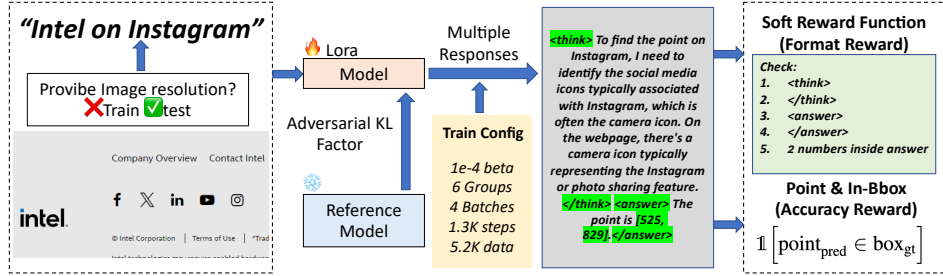
Figure 3: The overview of GuirlVG.
