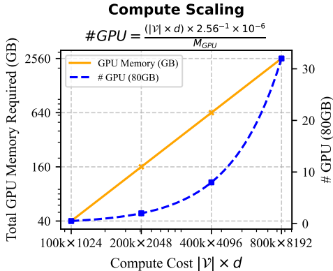
Figure 4: Compute scaling of G-reasoner.
