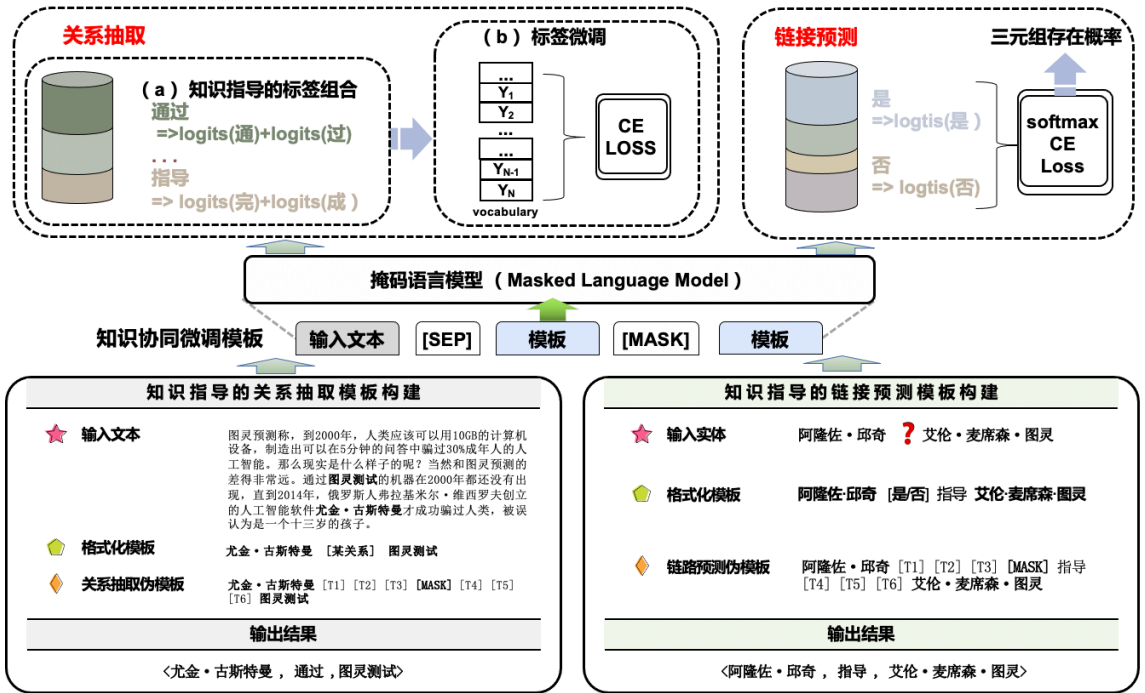
Fig.2 Knowledge collaborative fine-tuning, where T_i and Y_i (learnable) are unused or special tokens in the vocabulary. In this paper, the input text and template are fed into the masked language model. For link prediction, we estimate the probability of the triplet based on the output of the [MASK], and calculate the cross-entropy loss with the ground truth; for relation extraction, we convert the output of [MASK] to category labels based on the label mapping function, and calculate the cross-entropy loss with the ground truth.
