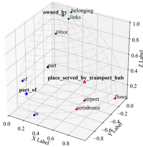
Fig.4 A t-SNE visualization of several relation representations learned in KnowCo-Tuning (optimized) on Wiki80 data
