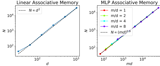
Figure 1: (Left) A linear associative memory can store N \propto d^2 associations. (Right) Empirically, the MLP associative memories can store N \propto (md)^{0.9} associations, approaching the N \propto md bound in Theorem 2. We attribute this discrepancy to challenges with the optimization dynamics.
