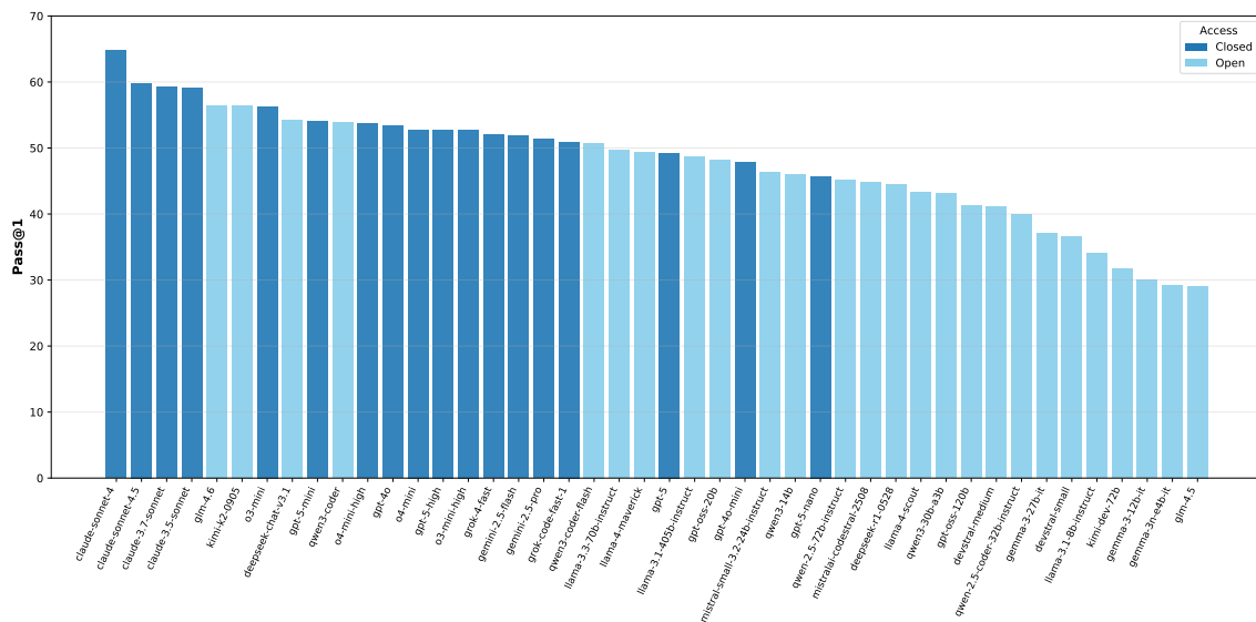
Figure 4: We evaluate 40 LLMs on EditBench. We report the pass@1 of each model; only 1 out of 40 models have a pass@1 greater than 60%. In general, closed-source models outperform open models.
