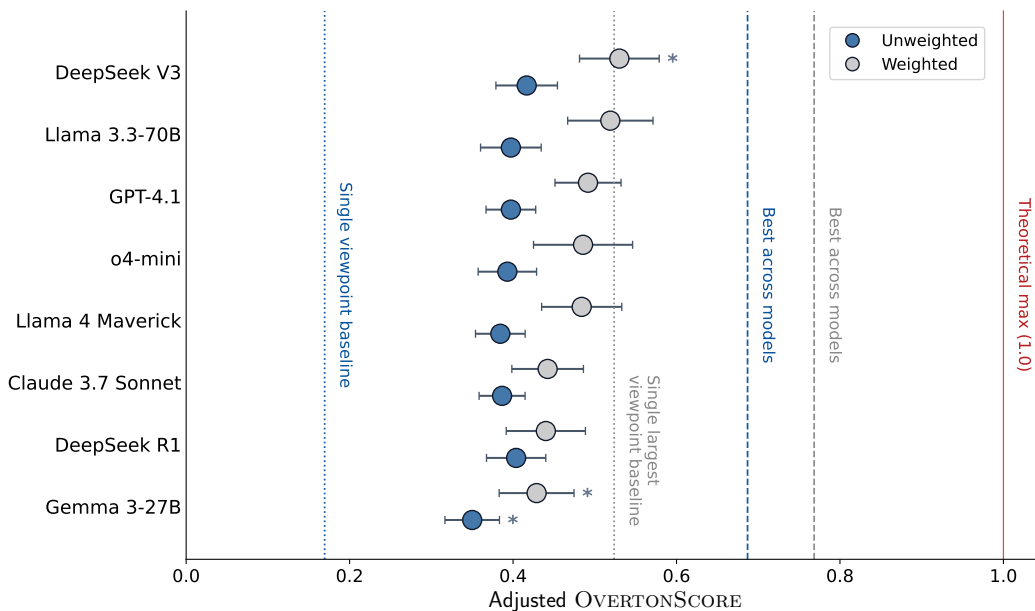
Figure 2: Benchmark results comparing the adjusted OVERTONSCOREs and weighted OVERTONSCORE W s with 95% question-level bootstrap CIs. An asterisk (*) denotes a statistically significant ( p < 0.05 ) difference from the mean. Note, both CIs and asterisks are comparable only within each metric variant.
