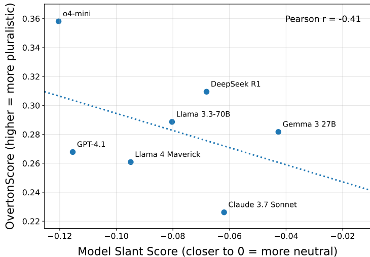
Figure 3: Comparison of Overton pluralism and political slant for the seven models and 15 questions appearing in both our benchmark and the Model Slant dataset. Higher OVERTONSCORE indicates more pluralistic representation; slant scores closer to 0 indicate higher perceived neutrality. Negative slant scores indicate bias towards Democrat views.
