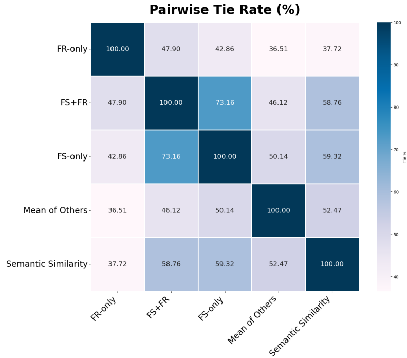
Figure 7: Tie rates for each method. To interpret the results, the tie rate is the proportion of the time the method in the row’s error equals the method’s error in the column. For example, Few-Shot+Free Response ties the semantic similarity baseline 58.76% of the time.
