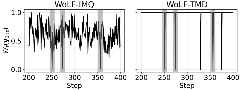
Figure 12. Trace of the weighting term for WoLF-IMQ and WoLF-TMD.
