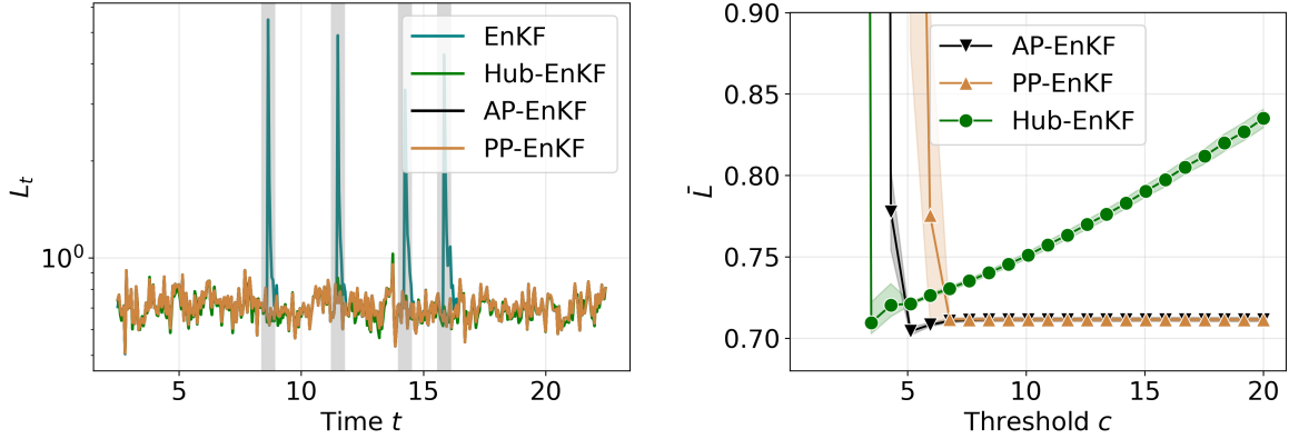
Figure 17. The left panel shows a run of the EnKF , the AP-EnKF , the PP-EnKF , and the Hub-EnKF ; with covariance inflation; outlier events are shown in grey vertical bars. The right panel shows the bootstrap estimate of L_T over 20 runs and 500 bootstrapped samples as a function of the c hyperparameter.
