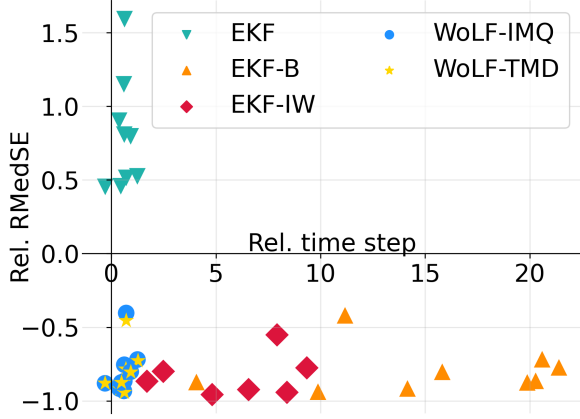
Figure 5. RMedSE versus time per step (relative to the OGD minus 1) across the corrupted UCI datasets.
