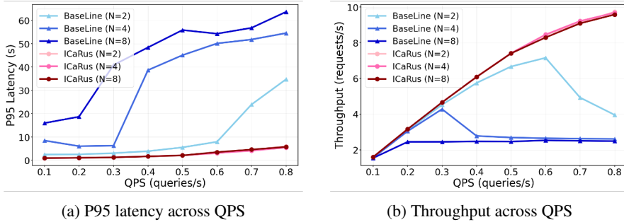
Figure 4: P95 latency and throughput of ICArus compared with multiple task-specific agents finetuned from the LLaMA-3.1-8B base model under the ReAct pattern. Here, N denotes the number of LoRA modules, which are integrated into multi model system built using either the conventional approach or ICArus.
