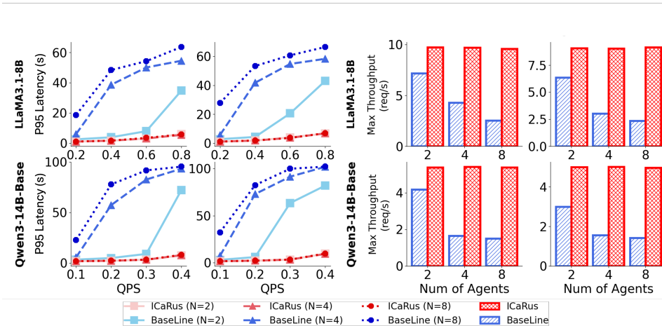
Figure 5: Comparison of P95 latency and maximum throughput across QPS for LLaMA3.1-8B and Qwen3-14B Base under ReAct and Reflexion patterns.
