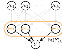
Figure 6: Markovian
