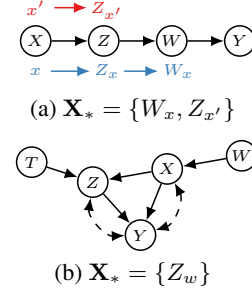
Figure 3: Invalid actions.
