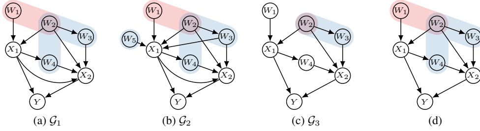
Figure 12: (a–c) Causal diagrams \mathcal{G}_1 , \mathcal{G}_2 and \mathcal{G}_3 ; red region represents w_1 and the blue one represents w_2 . Notably, ancestral relations are independent of confounders; (c) \mathcal{G}_3 with a realizable regime (valid action) when the value of W_2 is consistent; (d) Realizable regardless the value of W_2 .
