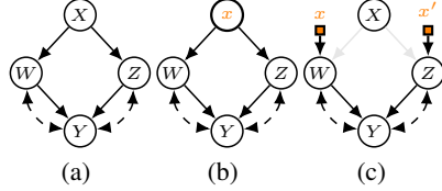
Figure 1: Counterfactual regime.
