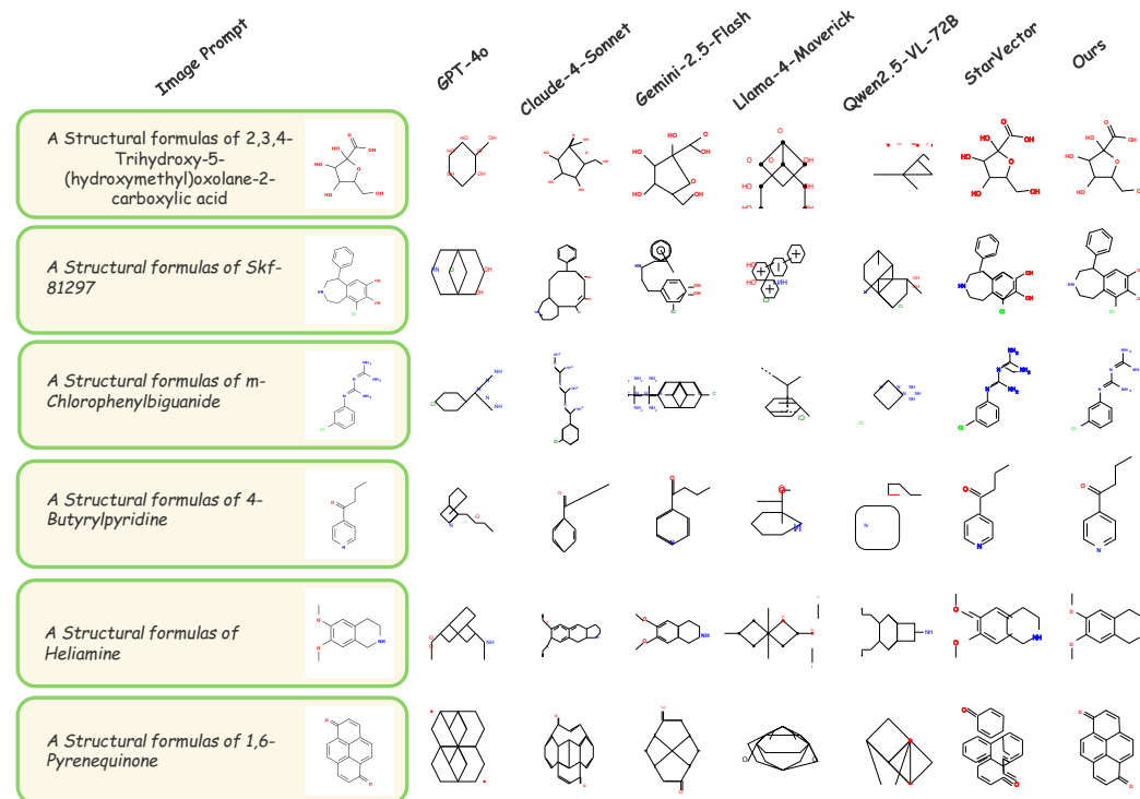
Figure 11: Qualitative comparison of Image-to-SVG performance between baselines and InternSVG on Sarena-Chemistry.
