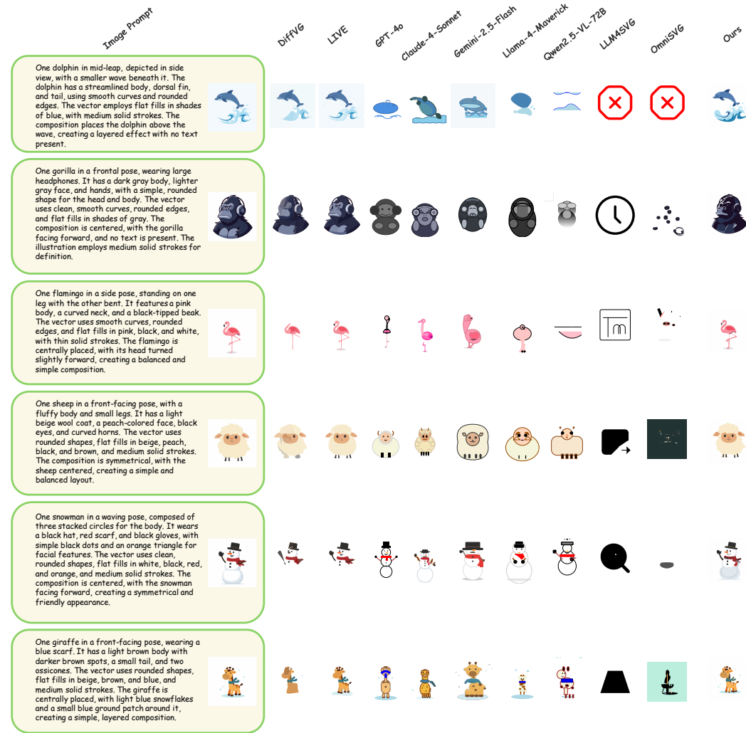
Figure 9: Qualitative comparison of Image-to-SVG performance between baselines and InternSVG on Sarena-Illustration. Red cross icons denote cases where the model failed to generate a valid SVG output.
