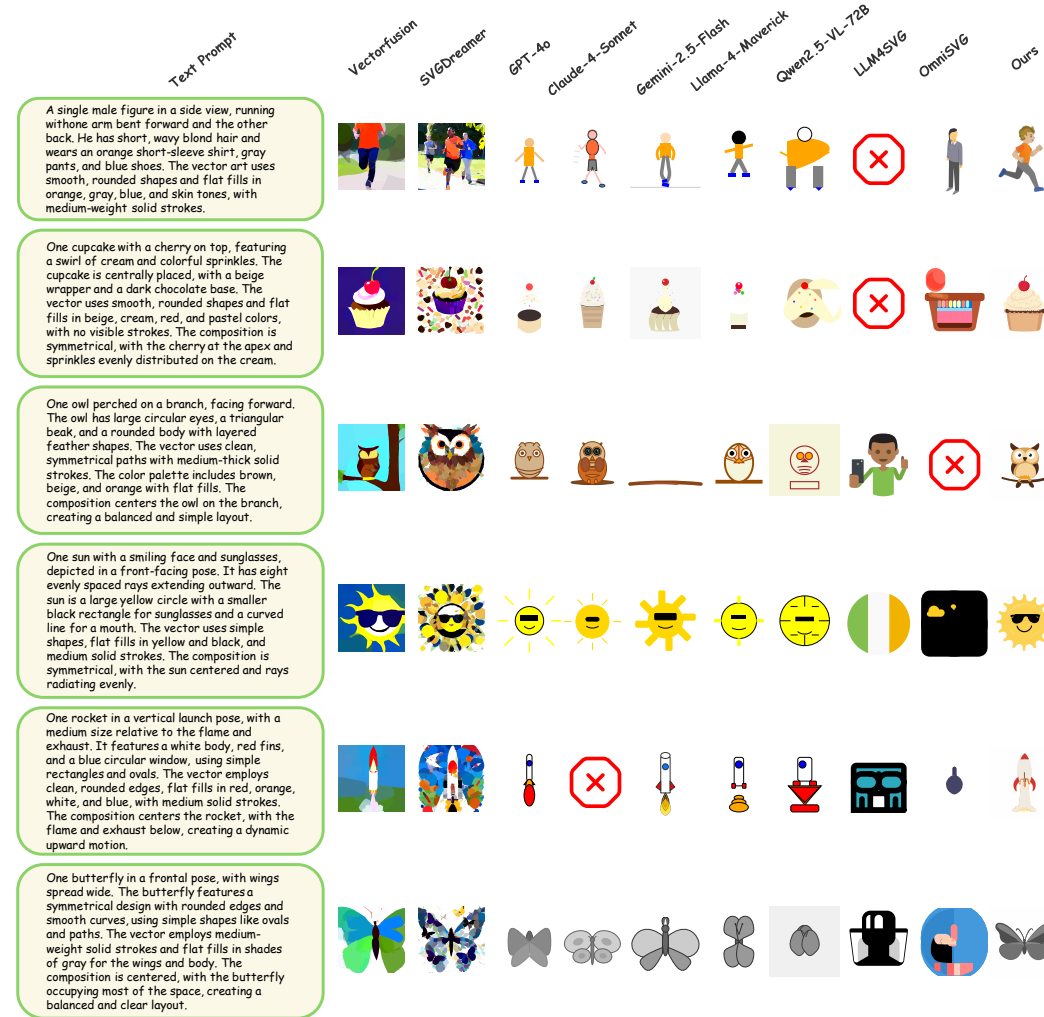
Figure 8: Qualitative comparison of Text-to-SVG performance between SOTA methods and InternSVG on SArena-Illustration. Red cross icons denote cases where the model failed to generate a valid SVG output.
