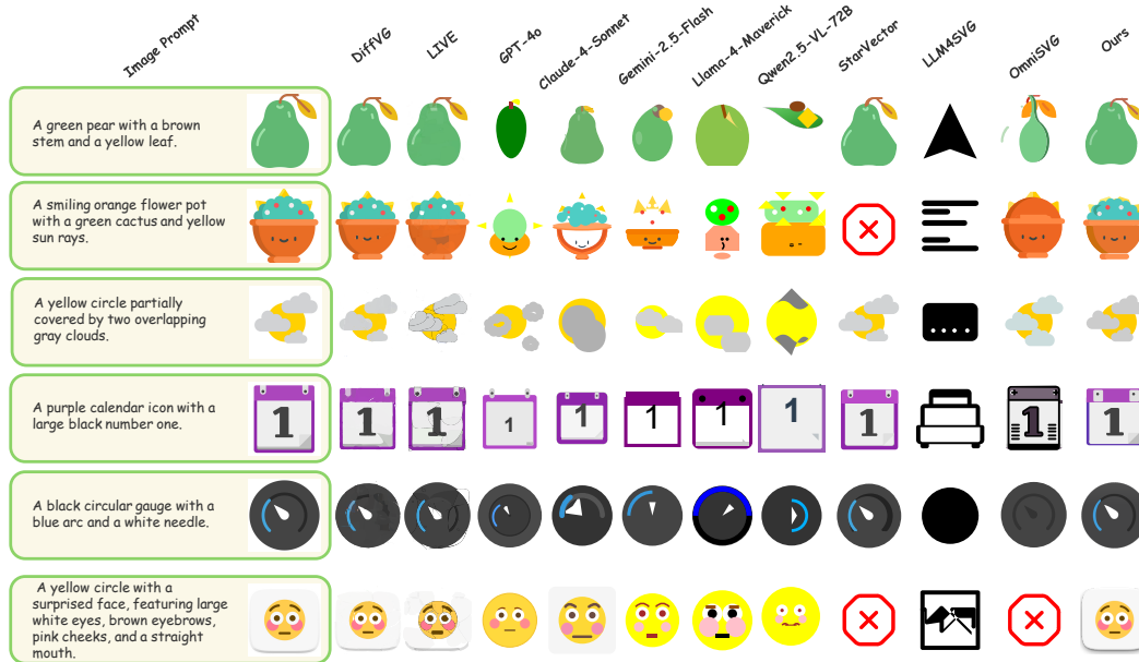
Figure 7: Qualitative comparison of Image-to-SVG performance between SOTA methods and InternSVG on Sarena-Icon. Red cross icons denote cases where the model failed to generate a valid SVG output.
