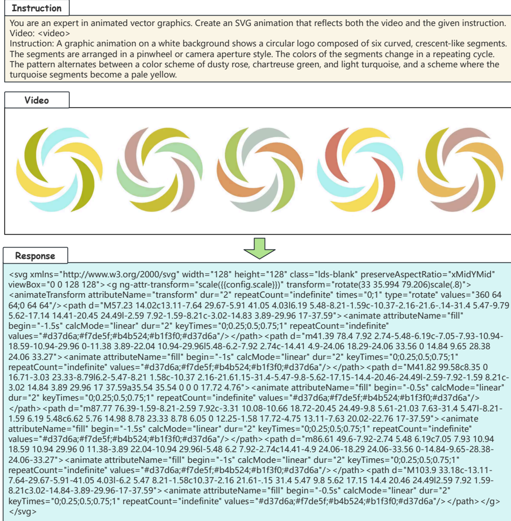
Figure 29: Examples of Video-to-SANI tasks.
