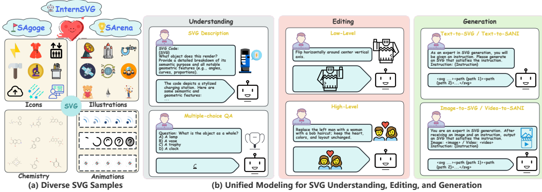
Figure 1: Overview of our InternSVG family. SAGoge provides large-scale and diverse SVG samples across multiple domains. SArena enables comprehensive assessment of existing MLLMs on SVG tasks. InternSVG supports unified modeling for SVG understanding, editing, and generation.
