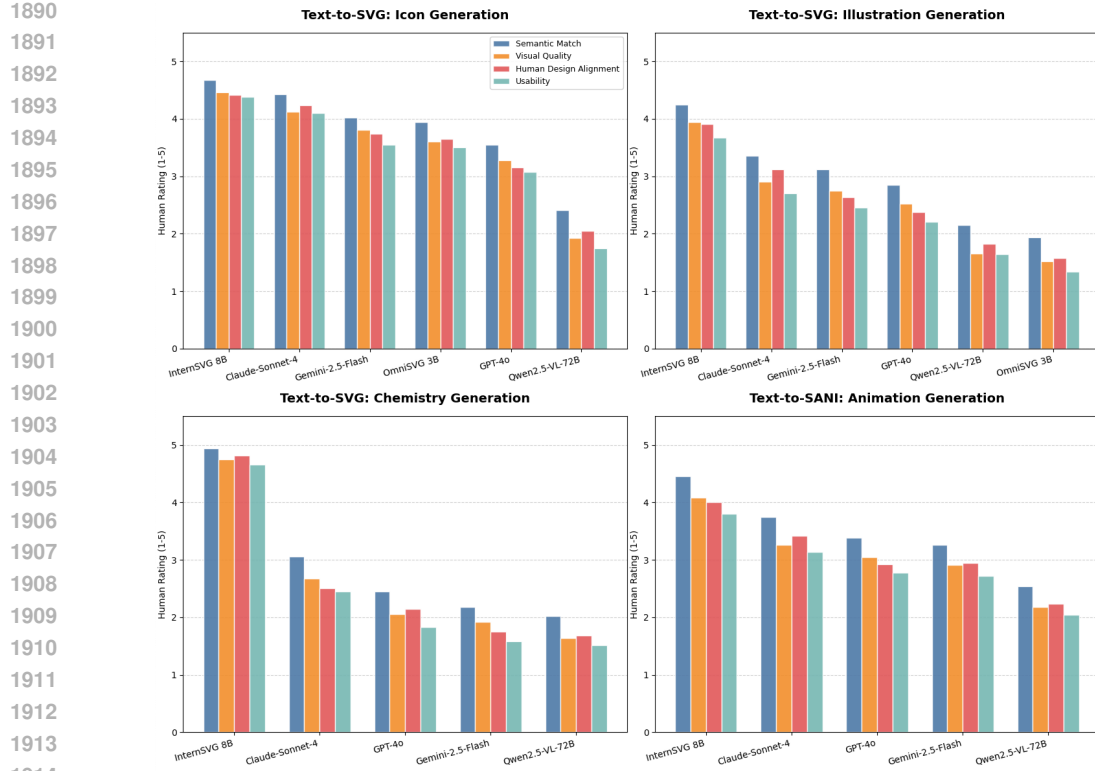
(a) Human evaluation results for Text-to-SVG / Text-to-SANI .
