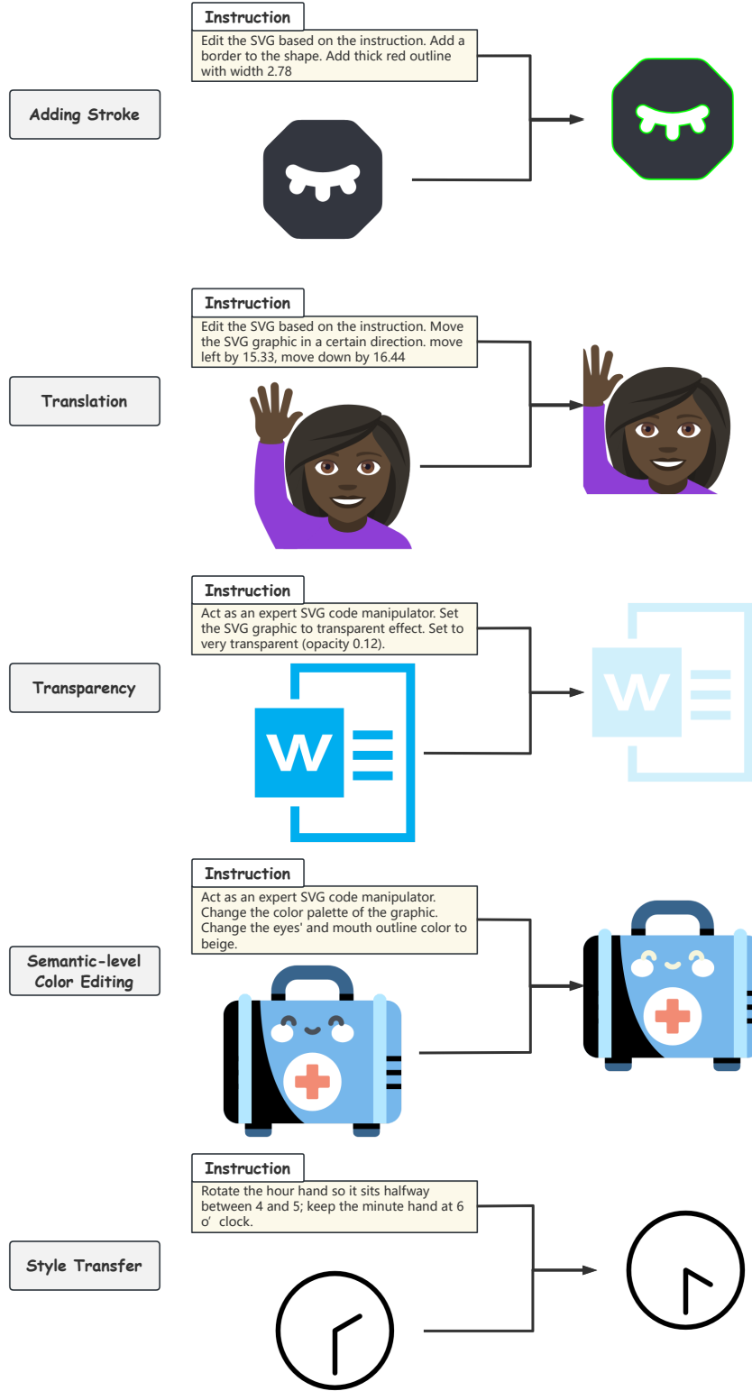
Figure 16: Visualization of InternSVG outputs on SVG editing.
