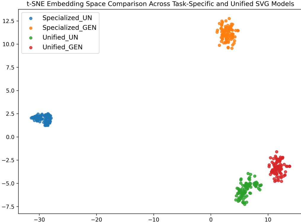
Figure 5: t-SNE visualization of model representations. Specialized models produce disjoint clusters for understanding and generation tasks, whereas the unified model yields neighboring clusters, revealing stronger cross-task representation coherence.
