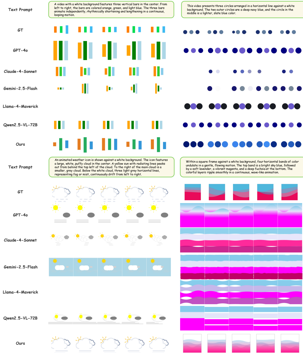
Figure 13: Qualitative comparison of Video-to-SANI performance between baselines and InternSVG on Sarena-Animation.
