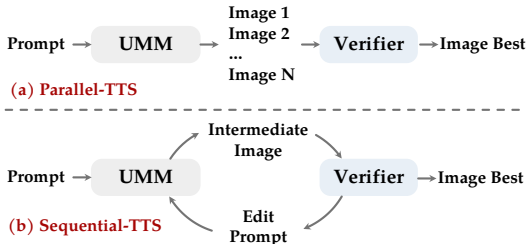
Figure 7: Comparison between Parallel and Sequential Test-Time Scaling.
