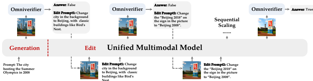
Figure 5: OmniVerifier-TTS: sequential test-time scaling pipeline of unified multimodal models.
