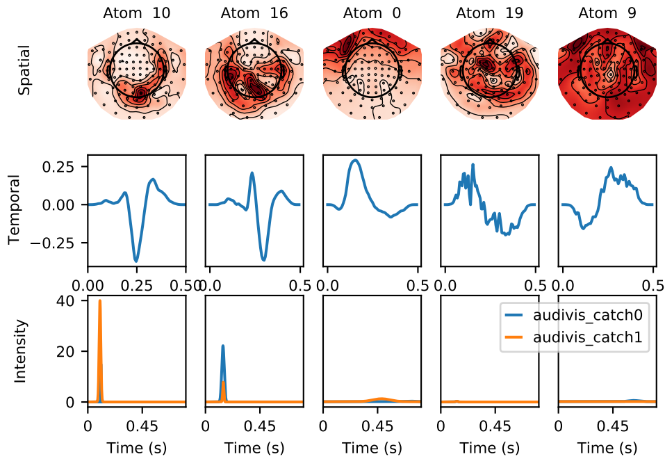
Figure A.11: Spatial and temporal patterns of the 5 atoms from Cam-CAN dataset subject CC620264, a 76.33-year-old female, and their respective estimated intensity functions following an audiovisual stimulus (cue at time = 0 s). Atoms are ordered by their bigger ratio \alpha/\mu .
