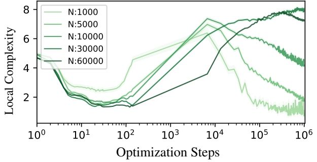
Figure 13. Memorization requirement delays grok. When training an MLP with varying number of randomly labeled MNIST samples, we see that with increase in the number of samples, the local complexity dynamics get delayed, especially the ascent phase gets elongated. This shows that with increased demand for memorization the network takes longer to complete ascent and later undergo region migration.
