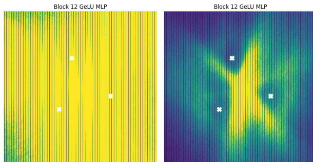
Figure 11. Token embedding space partition formed by the GeLU activated MLP of Block 12 of the GPT model mentioned in Figure 9. The partition is approximated by computing LC on a 512 \times 512 grid on a 2D subspace in the token embedding space. Note that after grokking (right), the three random samples used to determine the 2D subspace, has visibly lower local complexity in its immediate neighborhood.
