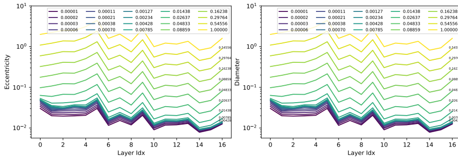
Figure 23. Change of avg. eccentricity and diameter (Xu et al., 2021) of the input space neighborhood by different layers of a ResNet18 trained on the CIFAR10 dataset, similar to the setting of Fig. 21. Resnet deforms the input neighborhood by reducing the avg. eccentricity and diameter of the neighborhood graphs. For r \leq 0.014 deformation is lower, indicating that smaller radius neighborhoods are reliable for LC computation on deeper networks.
