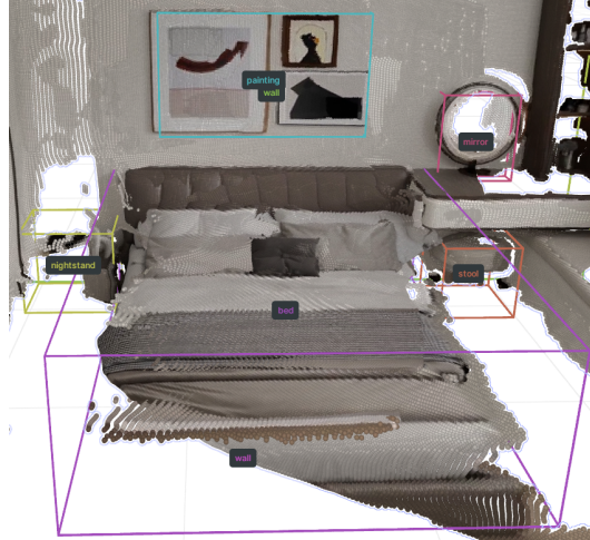
Figure 7: With a 0.8 merge rate, SpatialLM using our method still produces high-quality predictions.
