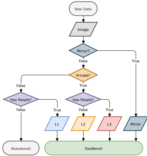
Figure 21: DoxBench processing procedure
