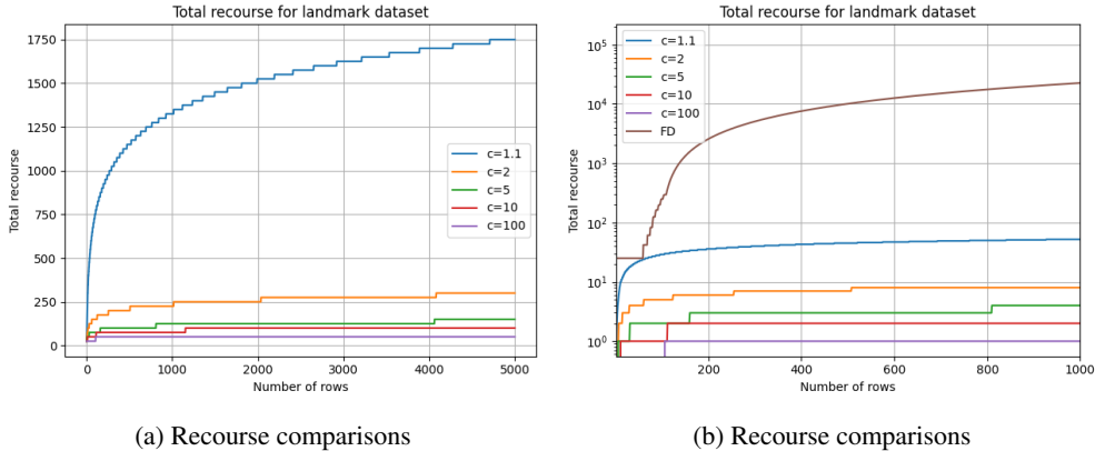
Fig. 1: Recourse comparisons for k = 25, c = (1 + \epsilon) \in \{1.1, 2.5, 5, 10, 100\}
