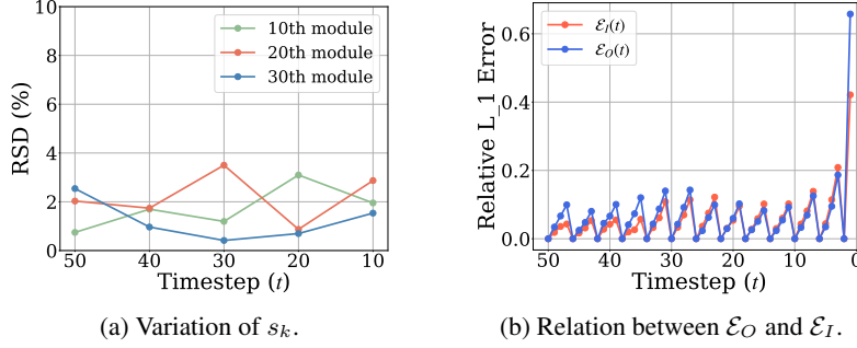
Figure 2: Empirical analyses in DiT-XL/2 (Peebles & Xie, 2023). (a) RSD of s_k(t - k) with varying t . (b) Relative L_1 errors of the output and input features, i.e. , \mathcal{E}_O(t) and \mathcal{E}_I(t) , respectively. Please see the text for details.
