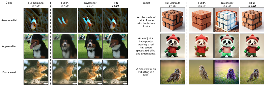
Figure 3: Qualitative comparisons of (left) class-conditional image generation for DiT-XL/2 (Peebles & Xie, 2023) on ImageNet (Deng et al., 2009), and (right) text-to-image generation for FLUX.1 dev (Batifol et al., 2025) on DrawBench (Saharia et al., 2022).
