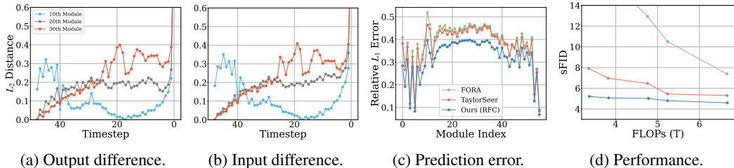
Figure 1: Feature analysis and comparison between existing approaches (FORA (Selvaraju et al., 2024), TaylorSeer (Liu et al., 2025b)), and our method (RFC) using DiT-XL/2 (Peebles & Xie, 2023). (a-b) Min-max normalized L_2 distances of output and input features, measured between consecutive timesteps. While the variations of feature changes are irregular, those of input and output remain closely aligned with each other. (c) The prediction errors across different modules. We measure the relative L_1 error between output features with and without applying caching methods and average the values over the timesteps. (d) Quantitative results on ImageNet (Deng et al., 2009) evaluated in terms of FLOPs and sFID (Nash et al., 2021).
