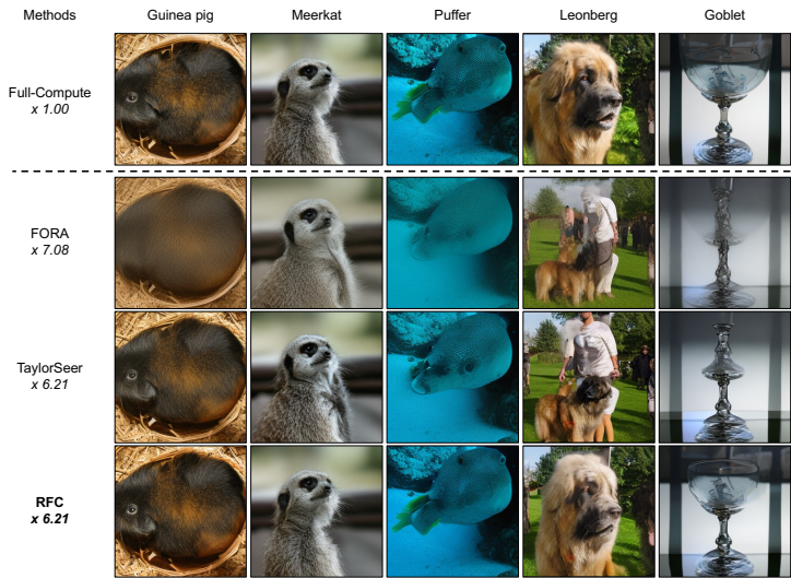
Figure 7: Qualitative comparisons of class-conditional image generation for DiT-XL/2 (Peebles & Xie, 2023) on ImageNet (Deng et al., 2009).
