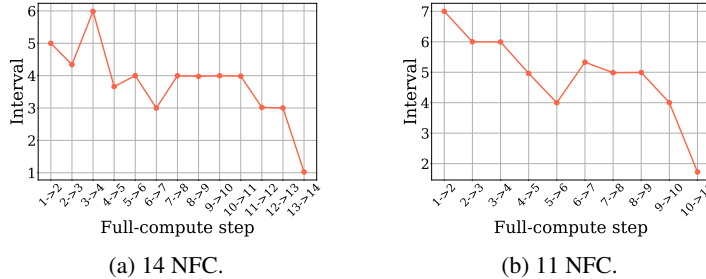
Figure 12: Analysis of non-uniform intervals scheduled by RCS using DiT-XL/2 (Peebles & Xie, 2023) on ImageNet (Deng et al., 2009). We visualize the average interval between full-compute steps for (a) 14 and (b) 11 NFC settings. i \rightarrow i + 1 at the x-axis denotes the i -th and (i + 1) -th full computation, and the y-axis shows the average interval. The results are averaged across 1,000 samples.
