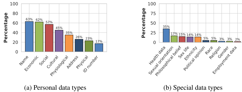
Figure 7: In contrast to OpenAI policies, ChatGPT memories store information which could be categorized as GDPR defined personal data or special category personal data.
