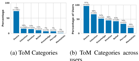
Figure 2: Distribution of memory entries among the different ToM categories as per GPT-4o annotations.
