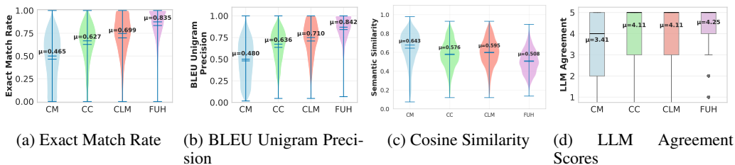
Figure 3: (a–b) Syntactic, (c) Semantic, and (d) LLM evaluation based provenance measures. Majority of ChatGPT’s memories are directly or semantically grounded in user input.
