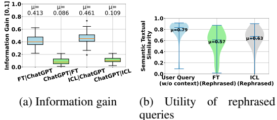
Figure 4: (a) Information gain of all predicted memories over ChatGPT memories shows high gain, hinting at higher potential risks. (b) Responses from rephrased queries from ICL and FT are semantically similar to the original response.
